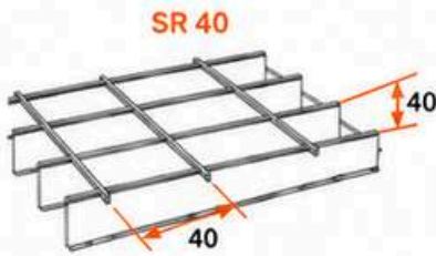
STANDARD GRATING SR 40
