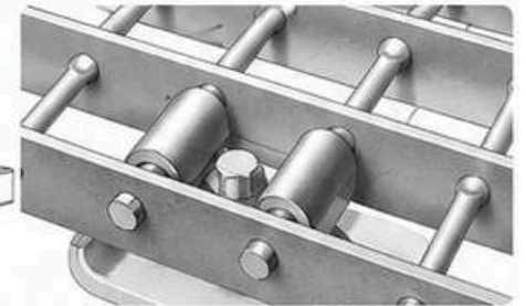
GRATING FASTENING METHOD
