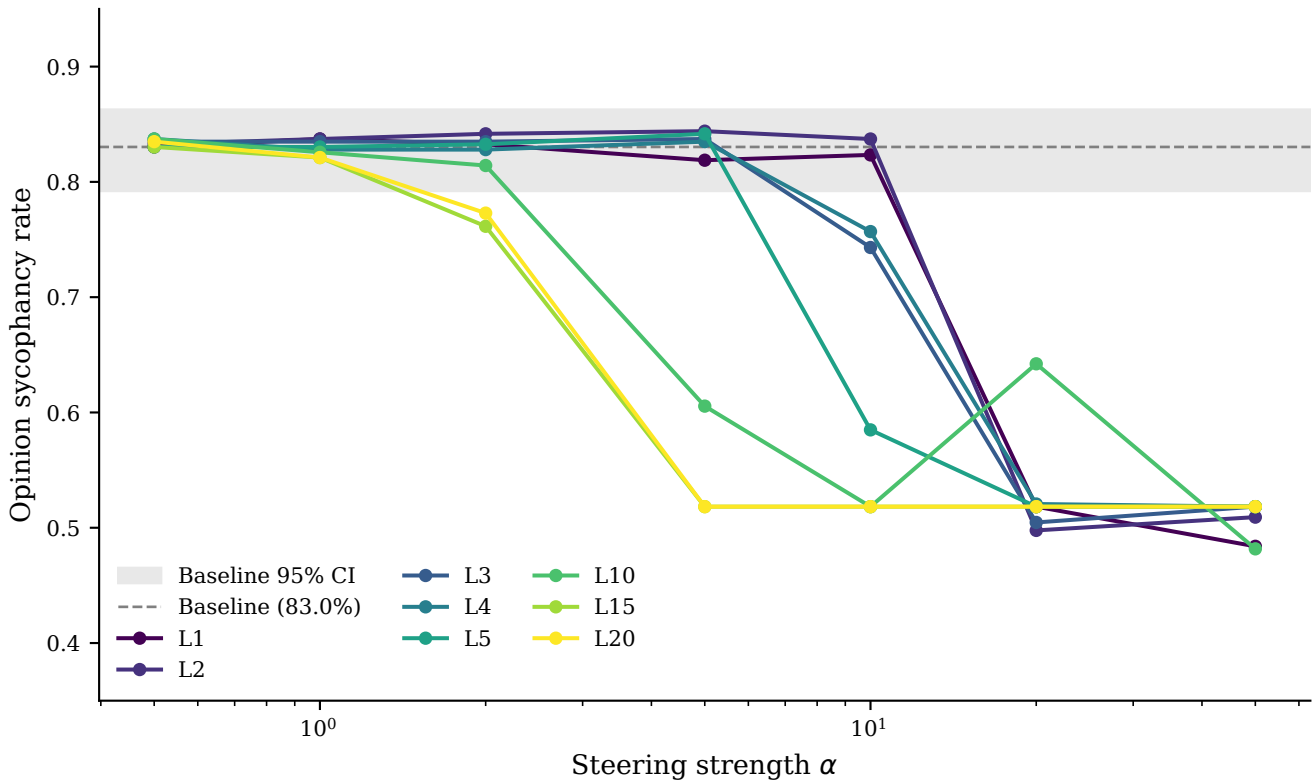
Opinion sycophancy vs. steering strength (per layer)
