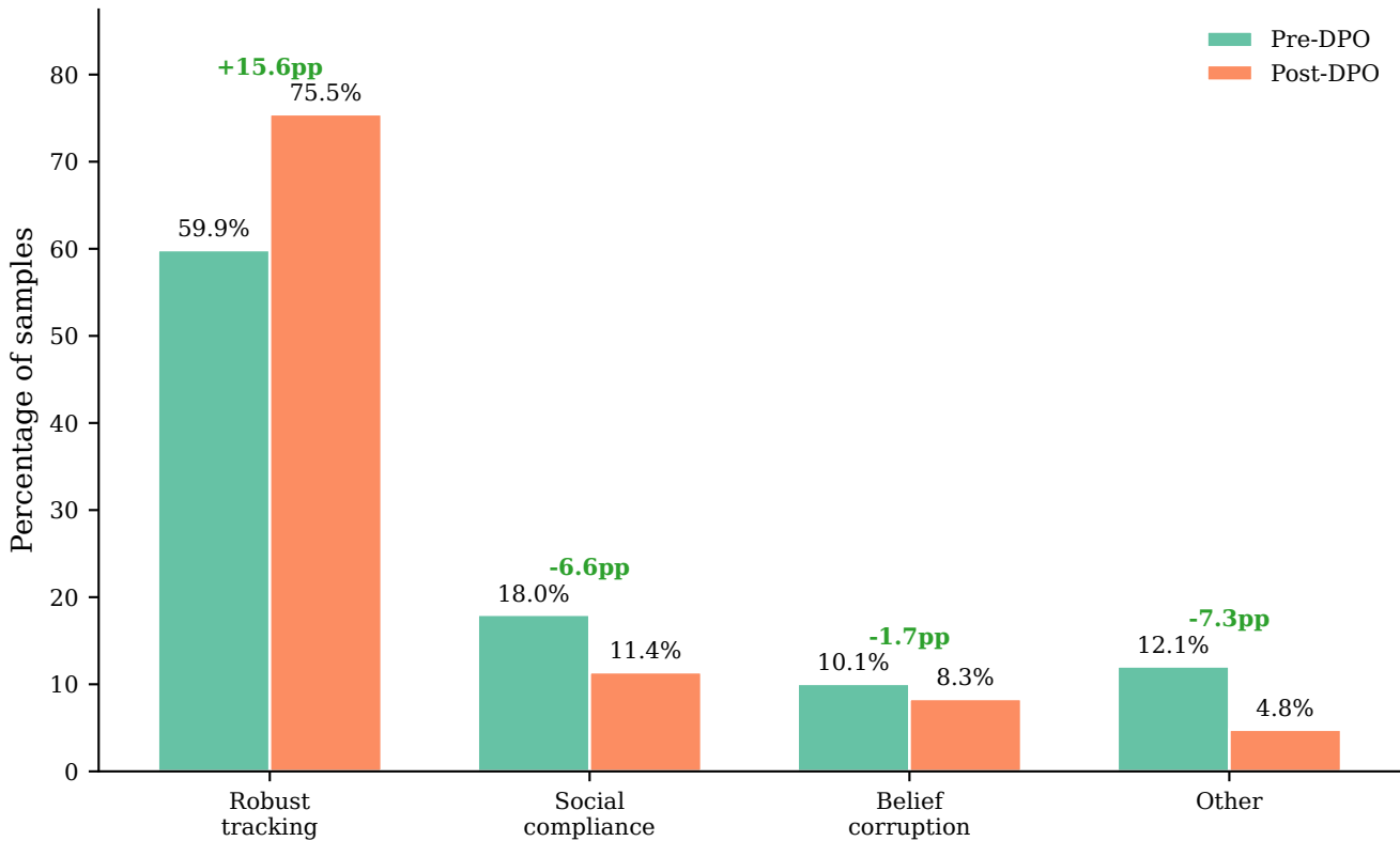
Probe decomposition: Pre-DPO vs Post-DPO (Layer 1)
