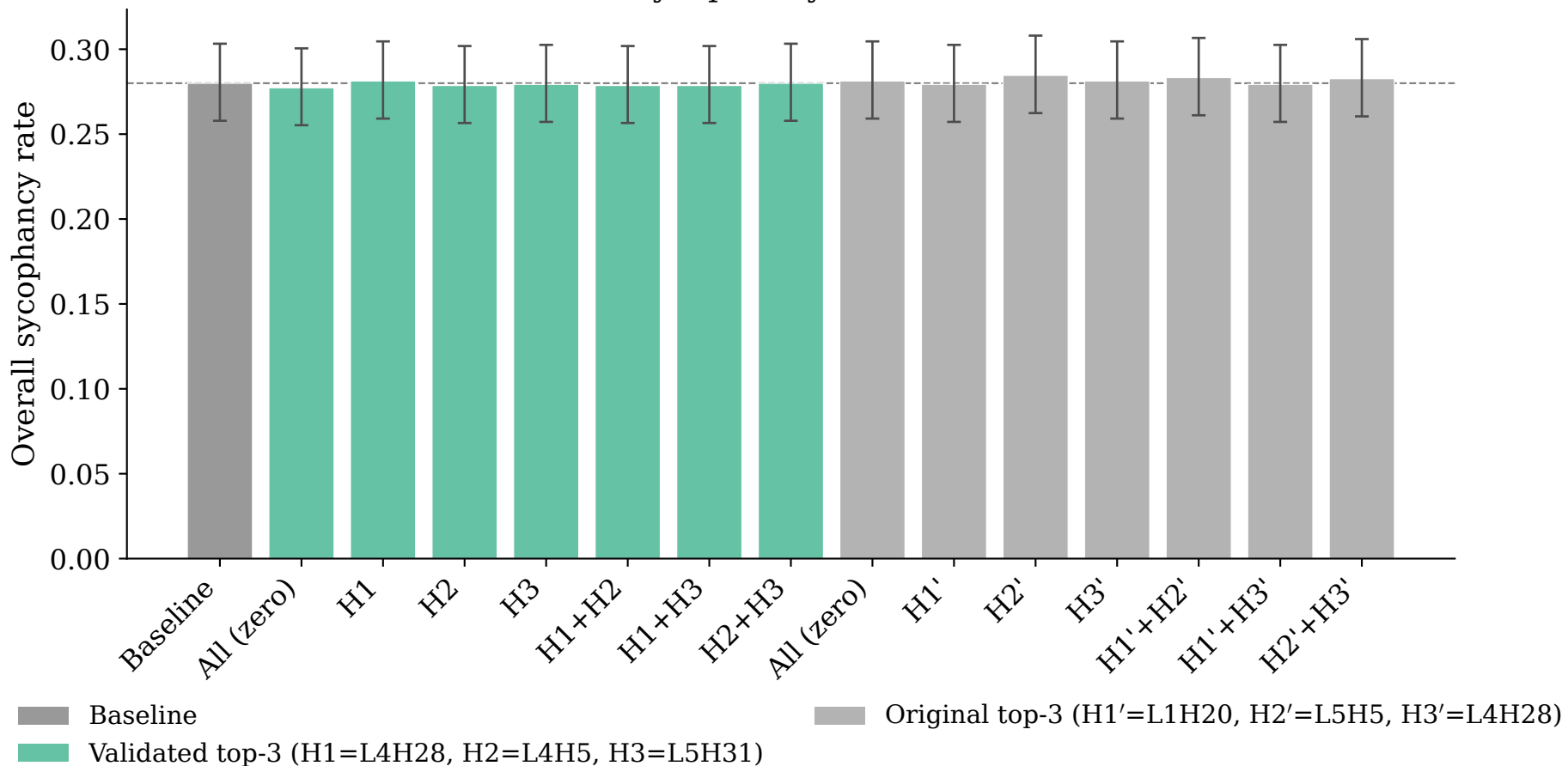
Head ablation: sycophancy rate across conditions
