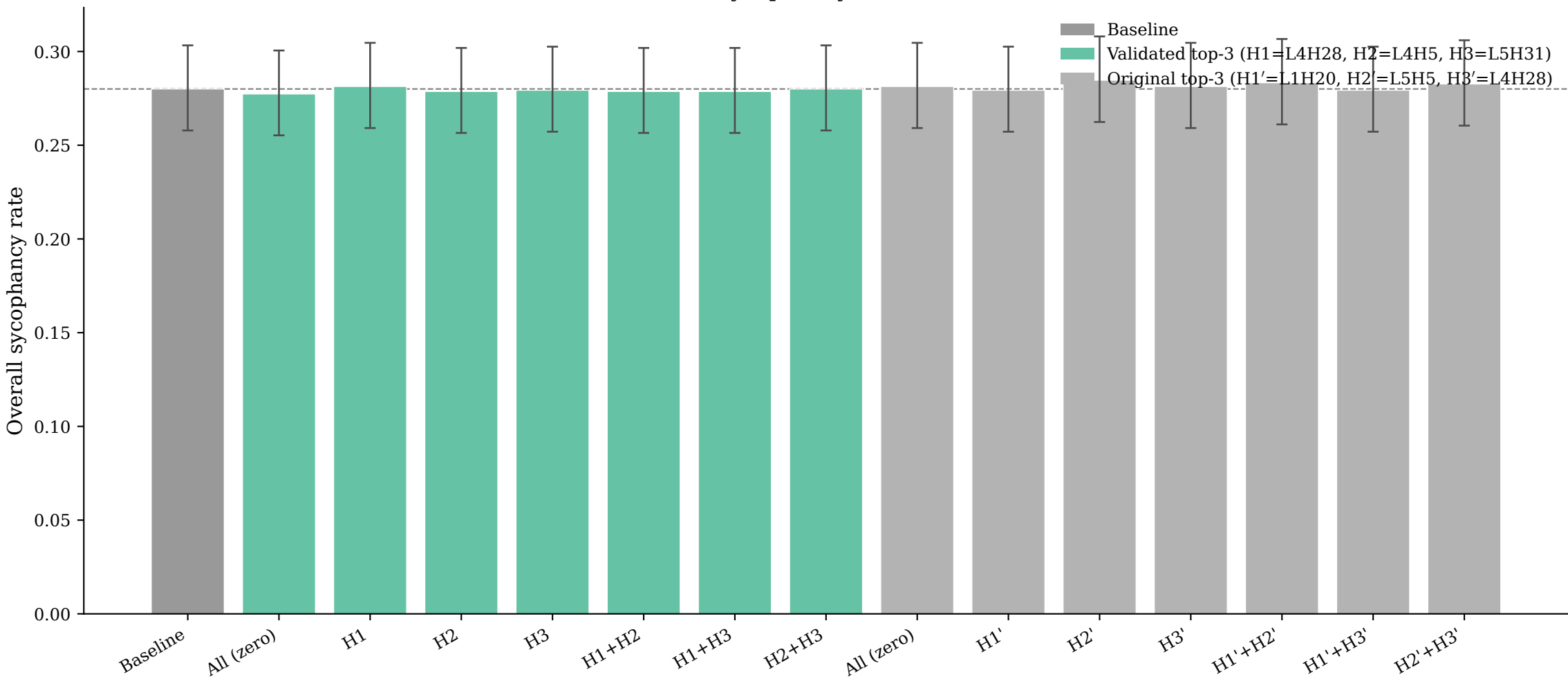
Head ablation: sycophancy rate across conditions
