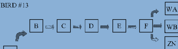
BIRD #13
