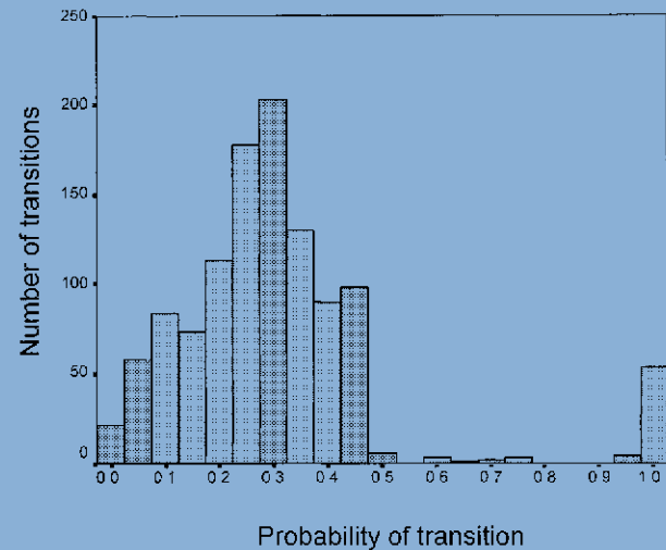
BIRD #117
