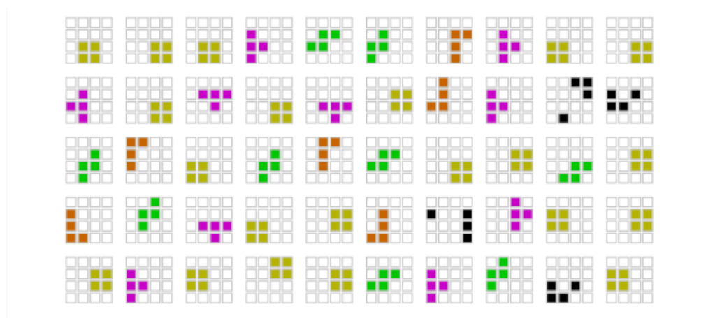
Chain 4, Generation 12
