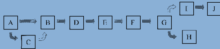
BIRD #117
