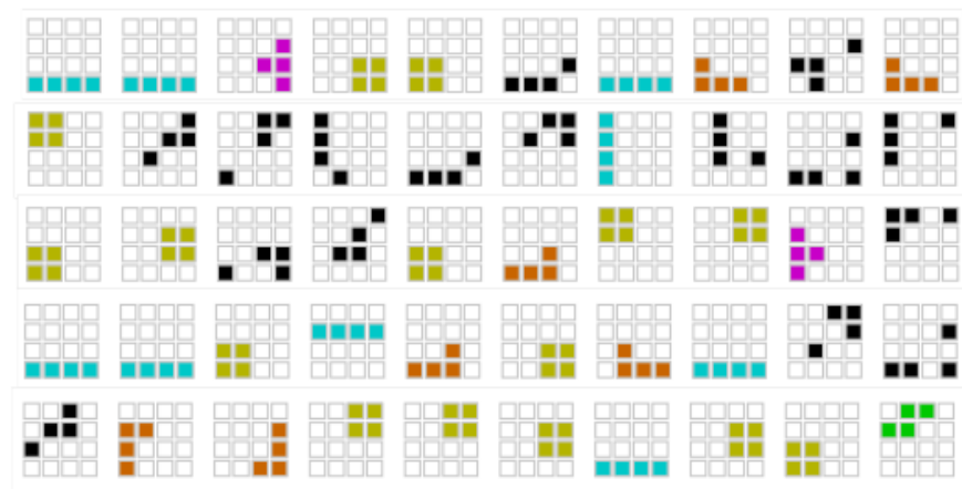
Chain 1, Generation 12
