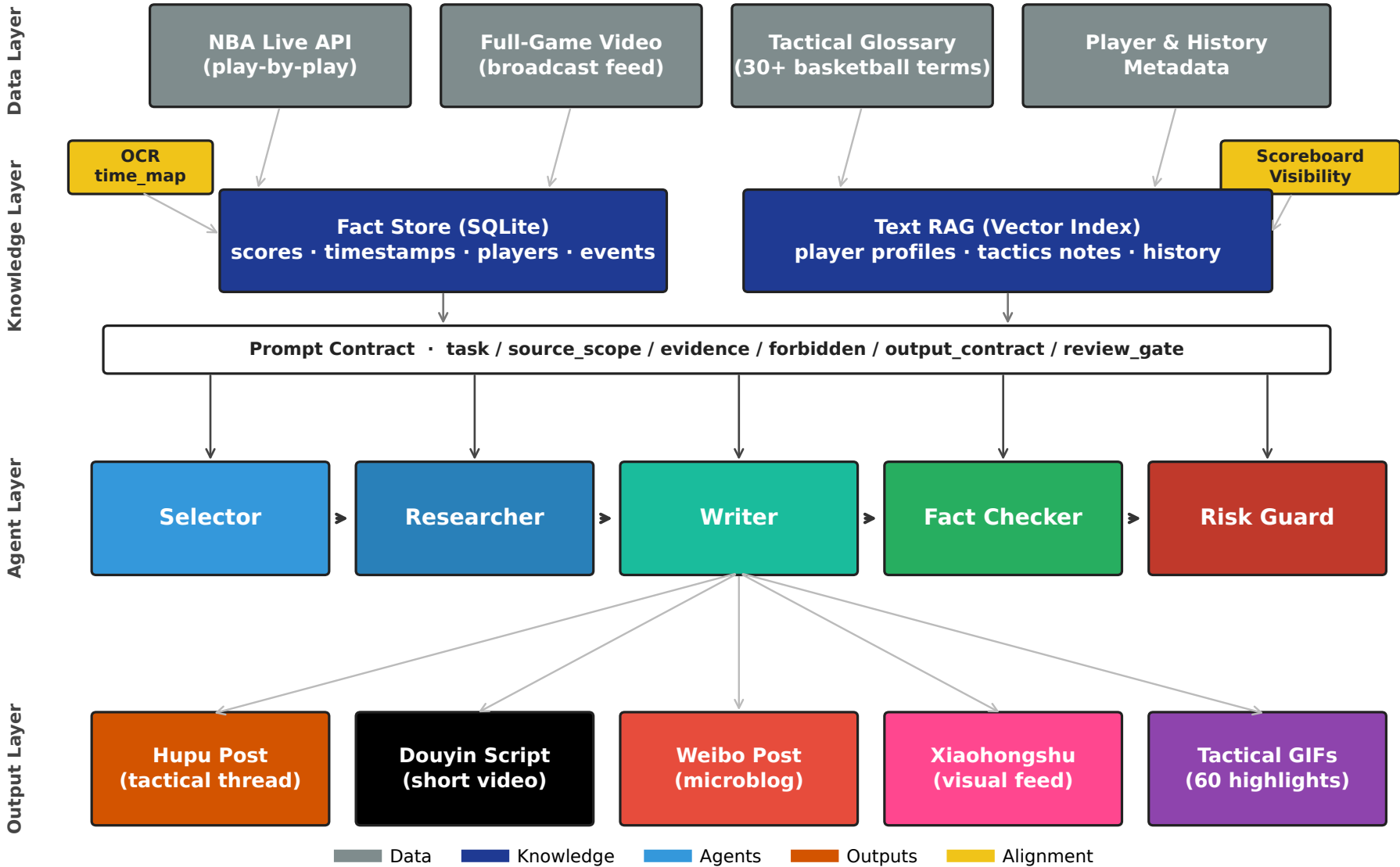
Figure 1. Multi-Agent Architecture for NBA Tactical Content Generation
