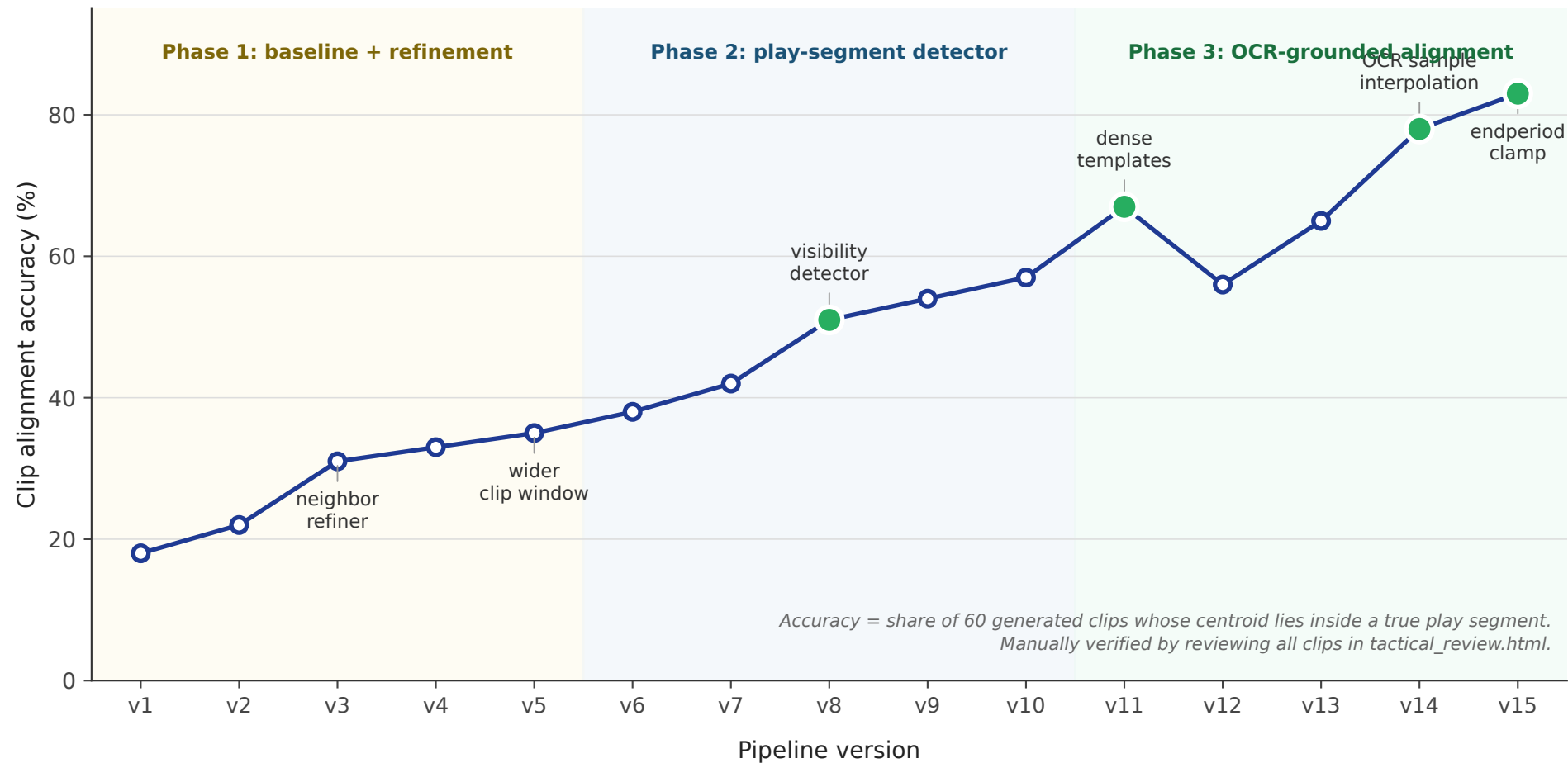
Figure 3. Clip-Alignment Accuracy across Pipeline Versions - OKC vs LAL G1
