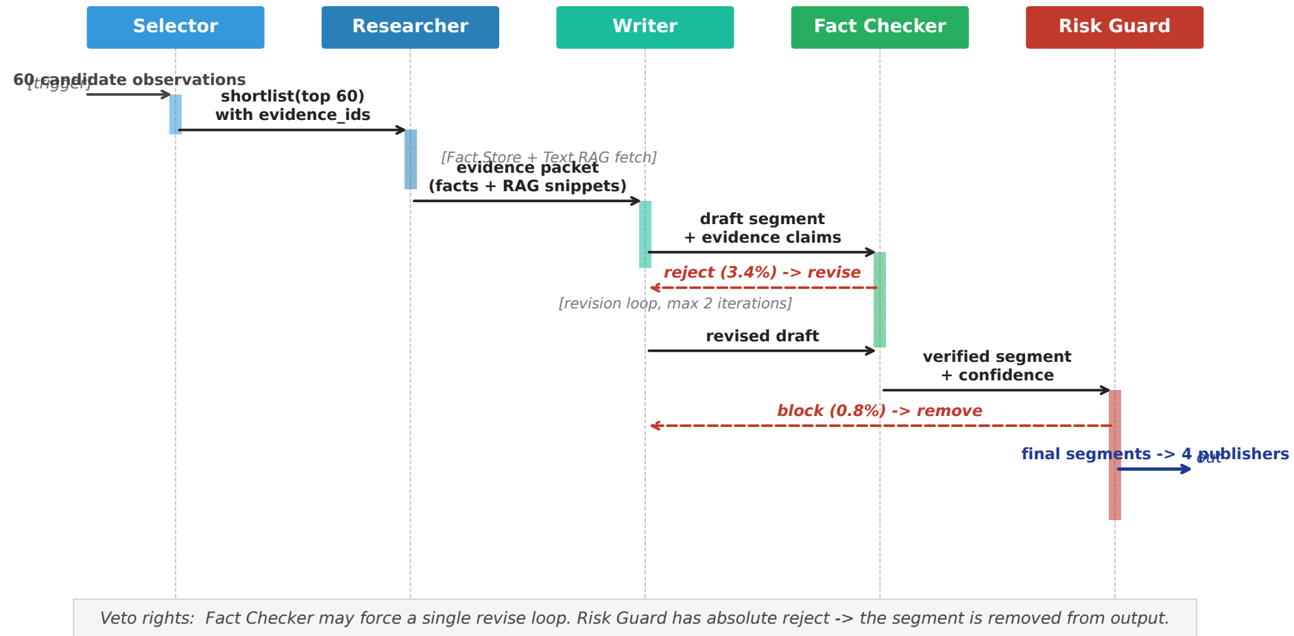
Figure 6. Five-Agent Supervision Protocol - Sequence Diagram
