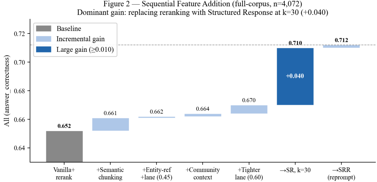
Figure 2: Sequential Feature Addition
