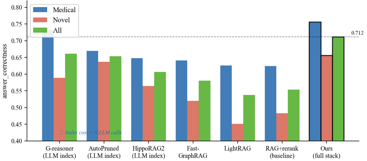
Figure 1 — GraphRAG-Bench Leaderboard (All systems use gpt-4o-mini judge; LLM index cost noted)
