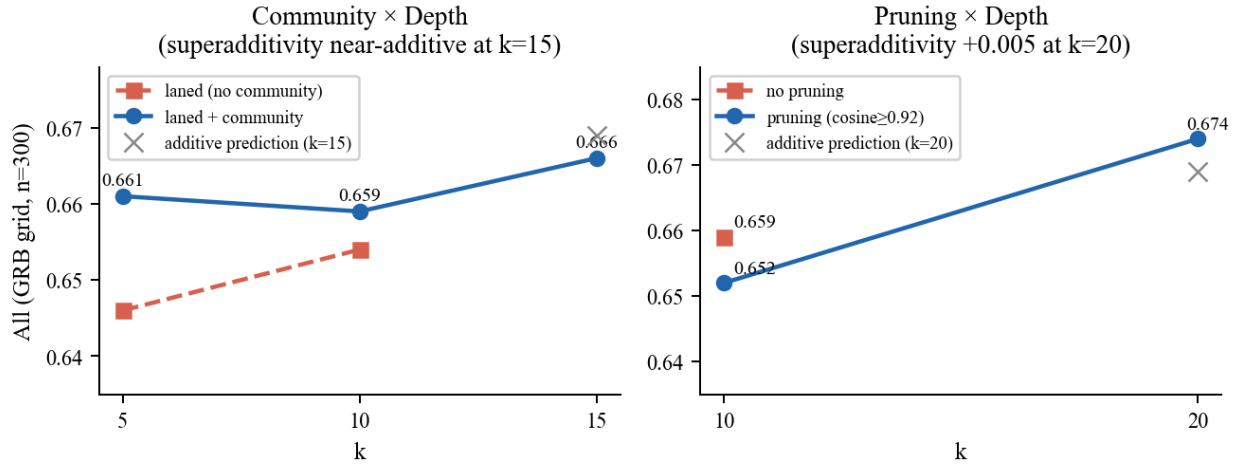
Figure 3: Community and Pruning Superadditivity
