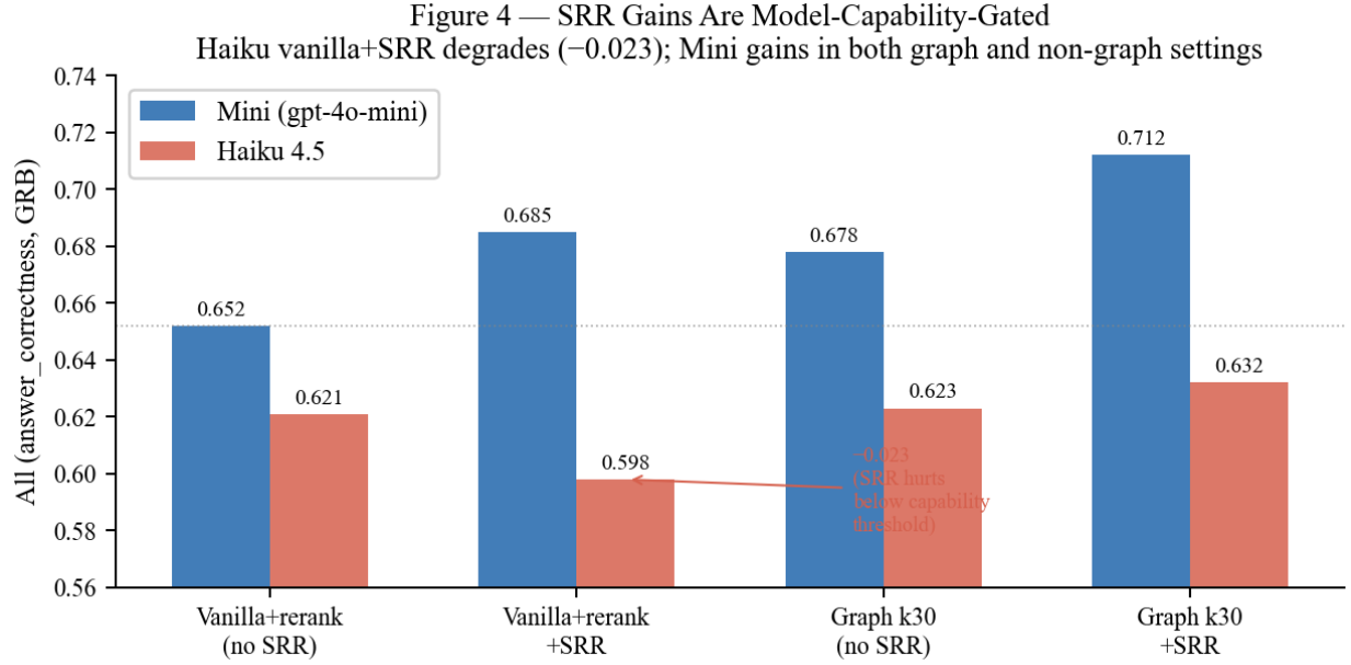
Figure 4: SRR Model Capability Gating
