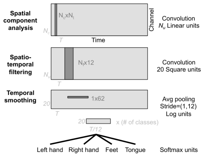
Fig. 1. The example architecture of SCCNet.
