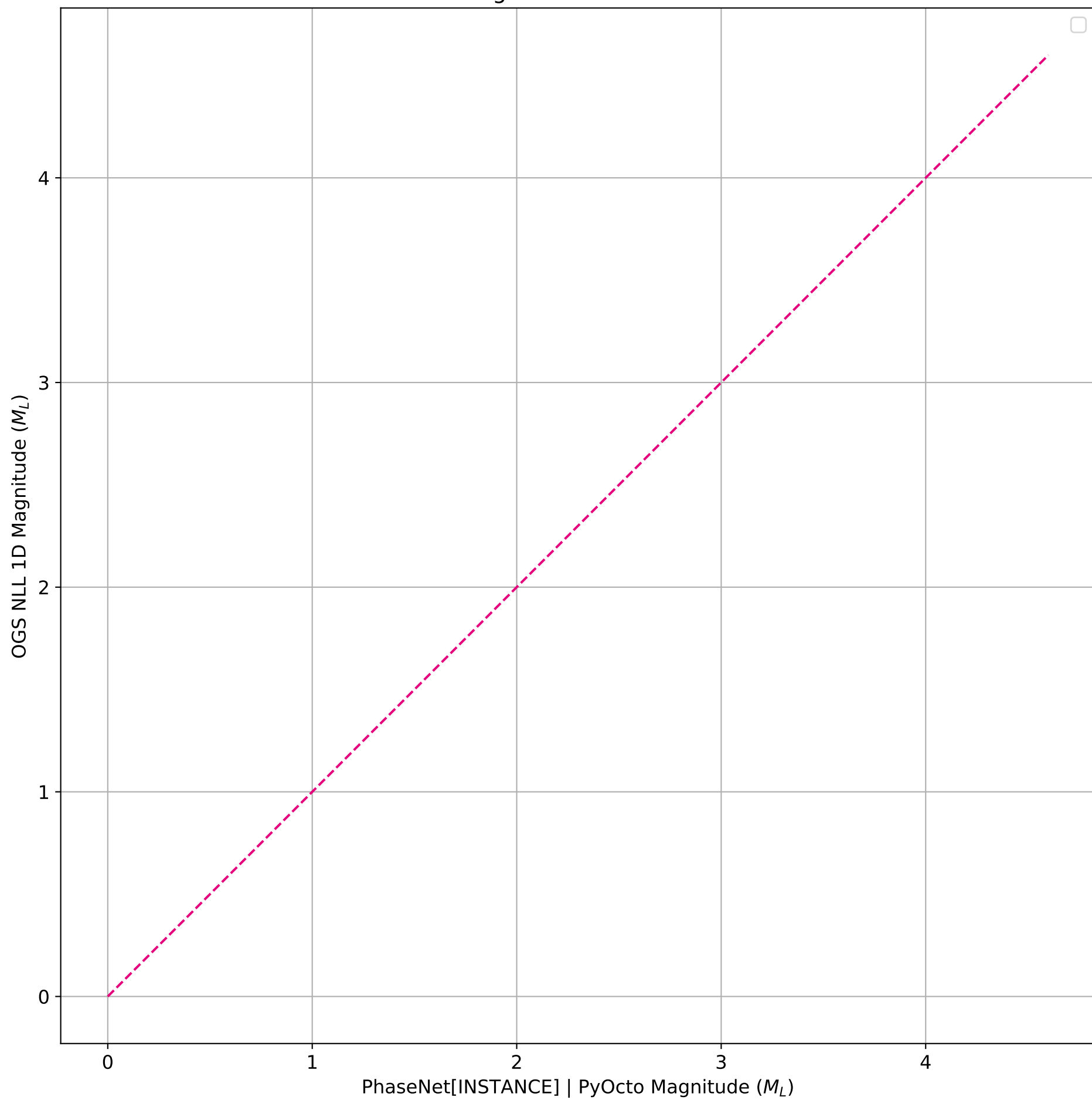
Magnitude Prediction
