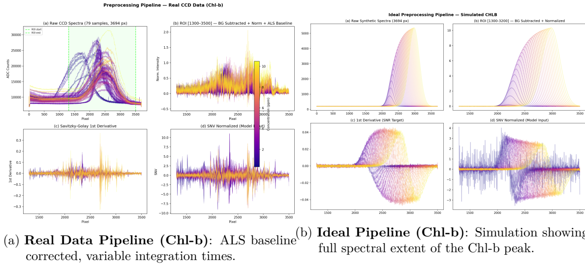
Figure 35: Chl-b Preprocessing Pipeline: Real Data vs. Simulation-Ideal.
