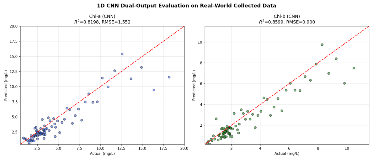
Figure 32: 1D CNN dual-output evaluation on real-world spinach-extract samples. The model captures the combined concentration trends despite limited training data.
