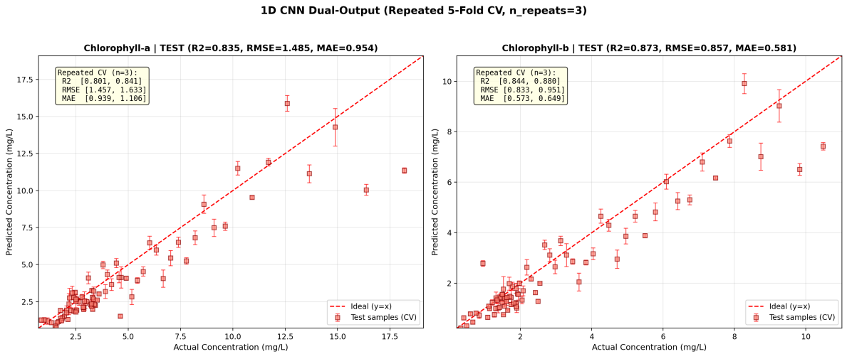
Figure 36: 1D CNN dual-output evaluation with Repeated 5-Fold CV (n=3). Red squares show mean predictions; error bars (1 ) quantify model stability. The summary boxes provide 95% CI bounds, showing comparable performance to the PLS baseline.
