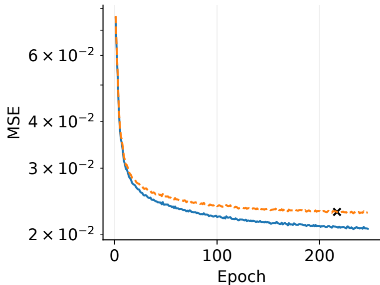
MNIST, width 64
