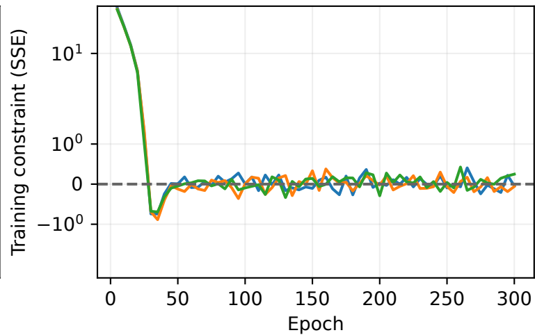
CIFAR-10
