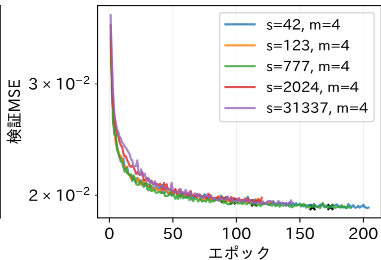
CIFAR-10
