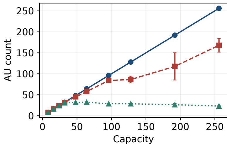
CIFAR-10
