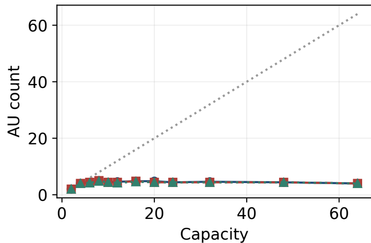
CIFAR-10
