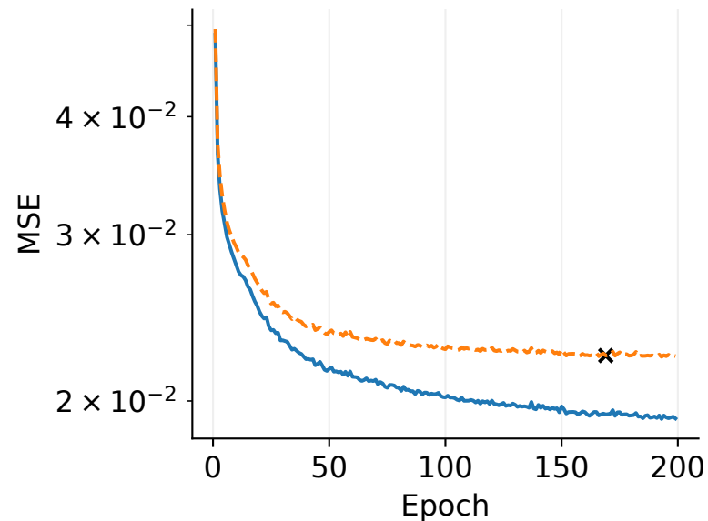
MNIST, width 6
