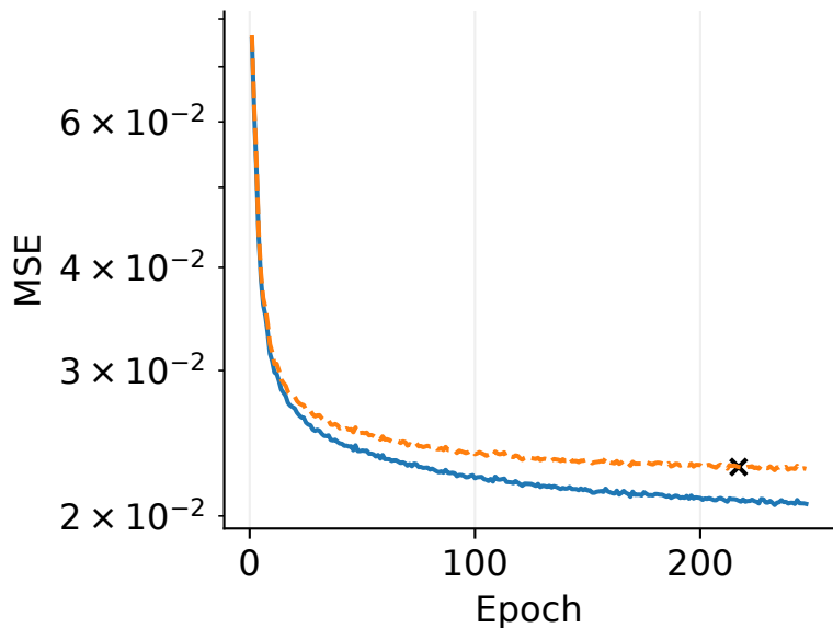
MNIST, width 64
