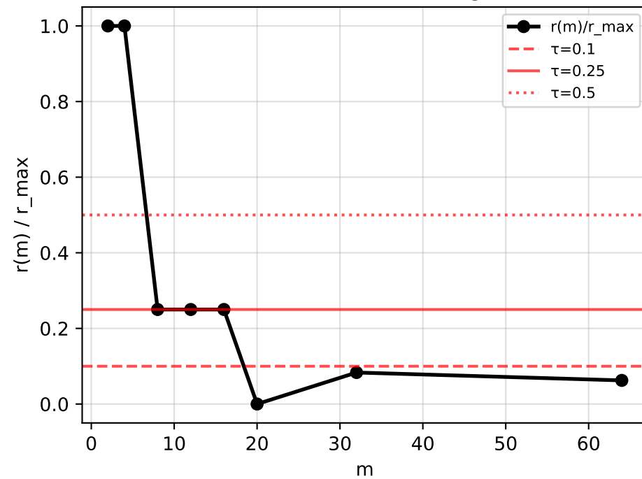
FashionMNIST: normalized AU growth rate
