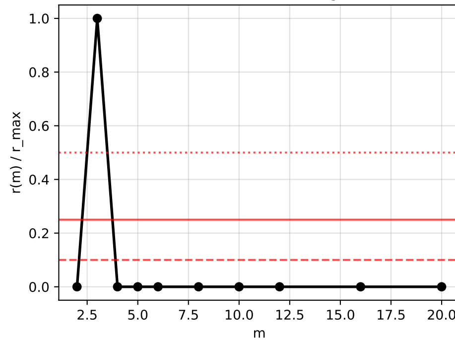
GaussianMix: normalized AU growth rate
