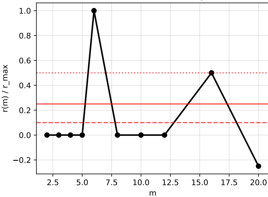
GaussianMix10: normalized AU growth rate
