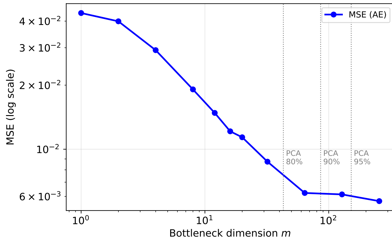
(a) AE: reconstruction MSE vs. m
