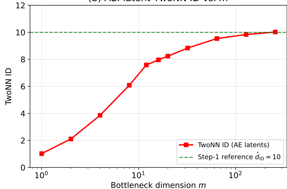
(b) AE: latent TwoNN ID vs. m
