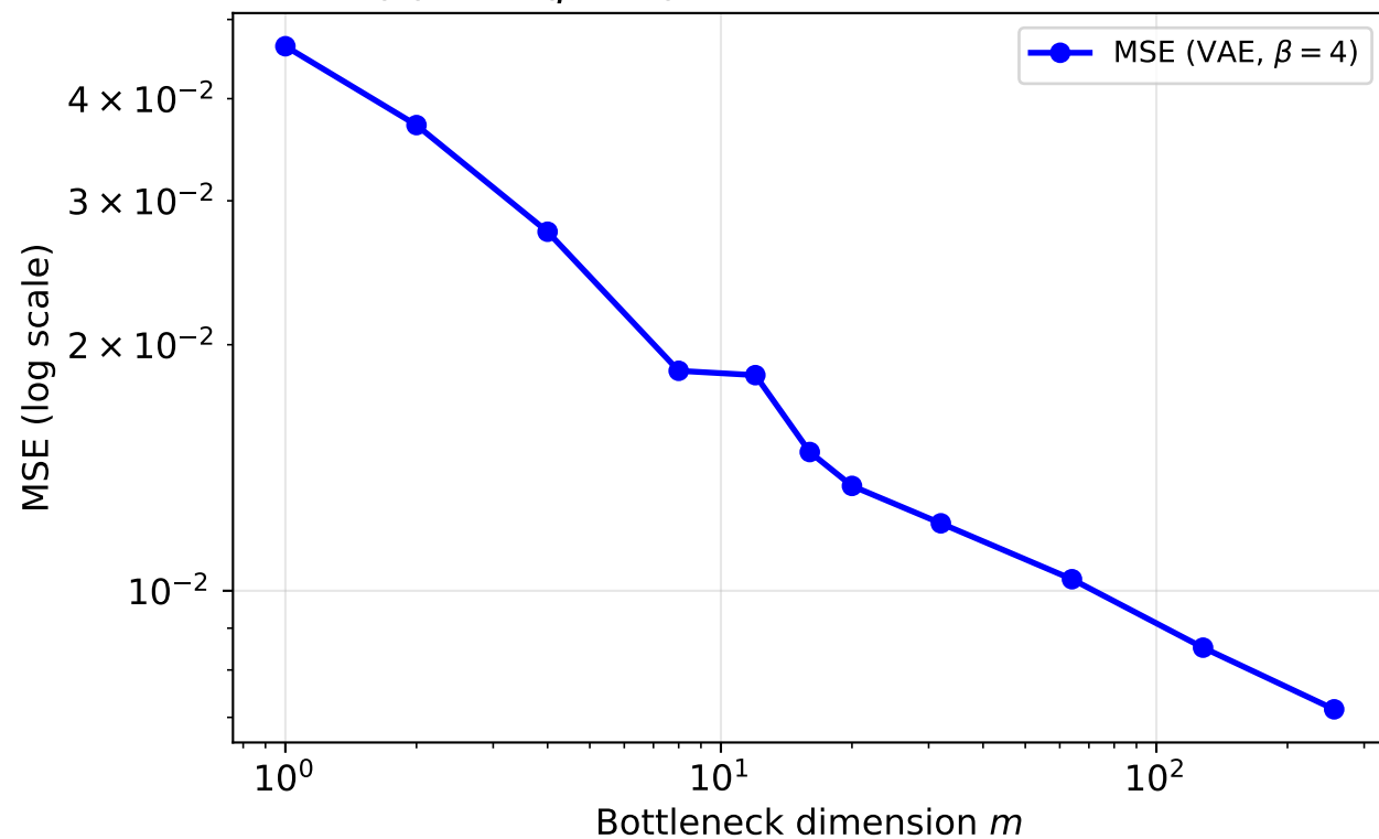
(c) VAE ( \beta = 4 ): reconstruction MSE vs. m
