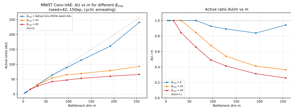
Figure 10. Exp-ConvV-HiBeta: Comparison of MNIST Conv-VAE AU vs m (left) and activation rate AU/m (right) for \beta_{\max} \in \{4, 10, 20\} . Increasing \beta_{\max} shifts AU saturation to lower dimensions, demonstrating the \beta -dependence of d^*(\beta) .
