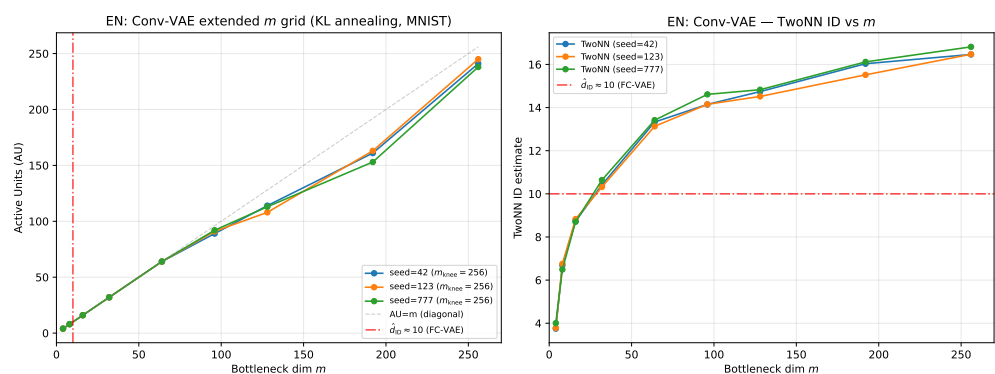
Figure 9. Exp-Conv-M256: Conv-VAE extended m grid ( m \in [4, 256] , KL annealing, 3 seeds). AU vs m (left) and TwoNN ID vs m (right). Diagonal line ( AU = m ) and FC-VAE reference \hat{d}_{\text{ID}} \approx 10 (red) are shown. AU = m continues at m \leq 64 but deviates from the diagonal at m \geq 96 , confirming qualitative water-filling behavior in Conv-VAE.
