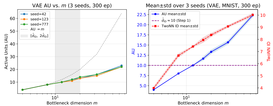
Figure 3. MNIST: multi-seed reproducibility of the AU verification signal (3 seeds, 300 epochs). Left: per-seed AU(m) with the ID-guided candidate range [d_{ID}, 2d_{ID}] shaded; right: mean±std band with the Step-1 reference \hat{d}_{ID} \approx 10 . AU values are highly reproducible ( \sigma \leq 0.5 ). Change-point (knee) estimates are deliberately not shown here; they are exploratory only (Appendix B).
