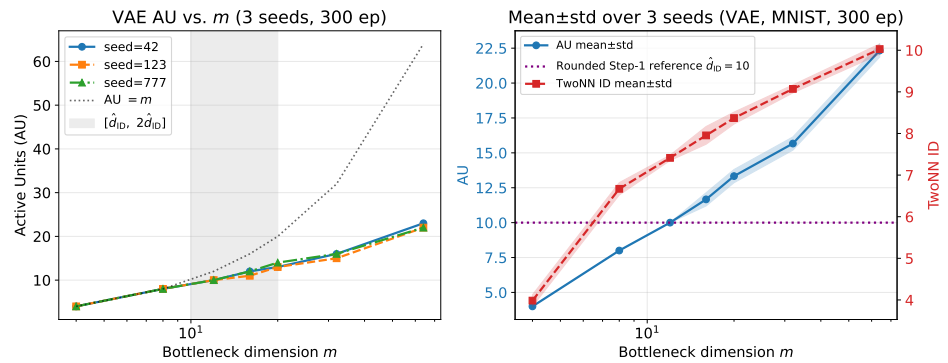
Figure 3. MNIST: multi-seed reproducibility of the AU verification signal (3 seeds, 300 epochs). Left: per-seed AU(m) with the ID-guided search window [d_{ID}, 2d_{ID}] shaded; right: mean±std band with the rounded Step-1 TwoNN reference \hat{d}_{ID} = 10 (an estimator-derived reference value, not a ground-truth dimension). AU values are highly reproducible ( \sigma \leq 0.5 ). Change-point (knee) estimates are deliberately not shown here; they are exploratory only (Appendix B).
