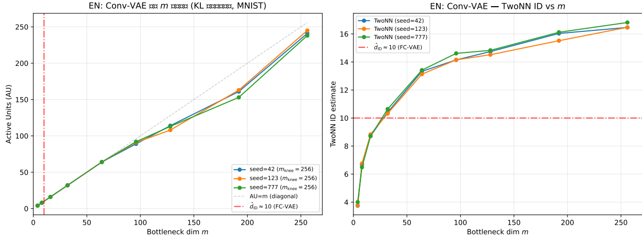
図 11: Exp-Conv-M256: Conv-VAE extended m grid ( m \in [4, 256] , KL annealing, 3 seeds). AU vs m (left) and TwoNN ID vs m (right). Diagonal line (AU= m ) and FC-VAE reference \hat{d}_{\text{ID}} \approx 10 (red) are shown. AU= m continues at m \leq 64 but deviates from the diagonal at m \geq 96 , confirming qualitative water-filling behavior in Conv-VAE. (Note: axis labels to be updated to English in final submission.)
