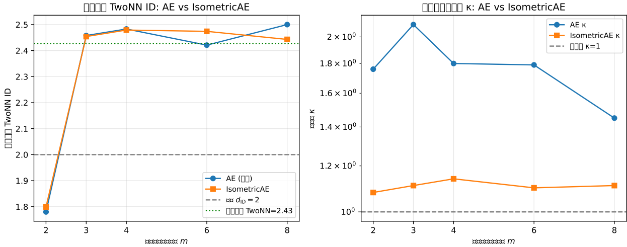
図 3: Exp-Iso-ID: (Left) Latent-space TwoNN ID by m — curves for standard AE and IsometricAE nearly overlap, showing that isometry improvement has minimal effect on TwoNN ID; (Right) Comparison of decoder condition number \kappa — IsometricAE maintains \kappa \approx 1.1 across all m , while AE rises to \kappa = 2.10 at m = 3 . (Note: axis labels to be updated to English in final submission.)
