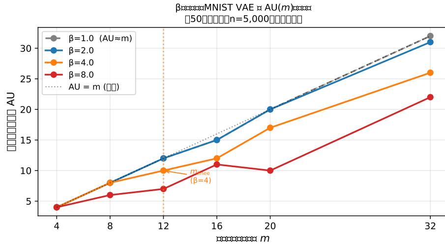
図 16: \beta -sensitivity analysis: AU vs m for MNIST VAE ( \beta \in \{1, 2, 4, 8\} , 50 epochs, subset). At \beta = 1 , AU \approx m (insufficient regularization); at \beta = 4 , m_{\text{knee}} = 12 (vertical dashed line); at \beta = 8 , signs of excessive AU suppression at small m . (Note: axis labels to be updated to English in final submission.)
