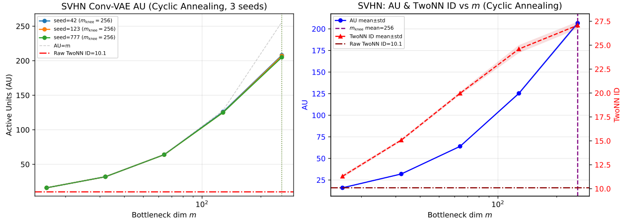
図 14: Exp-Nat-SVHN: m -dependence of AU and TwoNN ID for SVHN Conv-VAE (KL cyclic annealing, 3 seeds). (Note: axis labels to be updated to English in final submission.)
