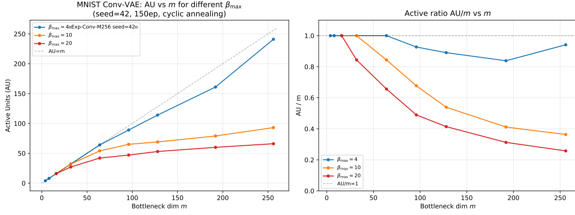
図 12: Exp-ConvV-HiBeta: Comparison of MNIST Conv-VAE AU vs m (left) and activation rate AU/m (right) for \beta_{\max} \in \{4, 10, 20\} . Increasing \beta_{\max} shifts AU saturation to lower dimensions, demonstrating the \beta -dependence of d^*(\beta) . (Note: axis labels to be updated to English in final submission.)
