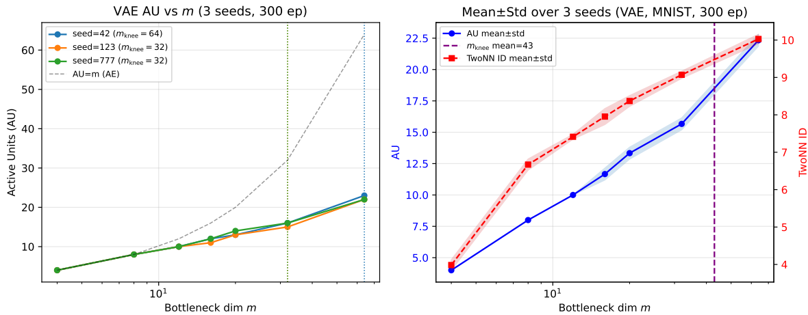
図 6: Exp-Mnist-Multi: AU patterns of MNIST VAE (3 seeds, 300 epochs). Left: AU vs m per seed (dotted lines: m^{\text{knee}} ); Right: mean \pm std band. AU and TwoNN ID bands are very narrow, but m^{\text{knee}} varies between 32 and 64 across seeds. (Note: axis labels to be updated to English in final submission.)
