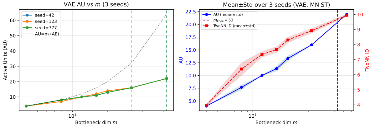
図 5: Exp-Mnist-Multi: AU patterns of MNIST VAE (3 seeds). Left: AU vs m per seed (dotted lines: m^{\text{knee}} per seed); Right: mean \pm std band. AU values are highly consistent across seeds, but m^{\text{knee}} varies between 32 and 64. (Note: axis labels to be updated to English in final submission.)
