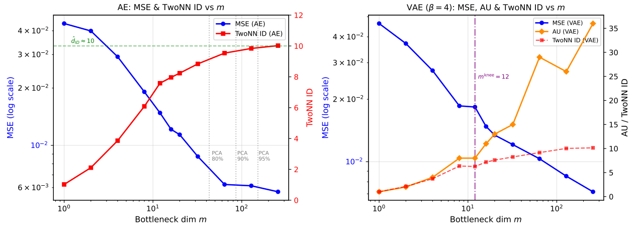
図 4: Exp-Mnist-Base: m -dependence of each indicator for MNIST (300 epochs). Left (AE) : MSE (log scale, left axis) and TwoNN ID (right axis). Vertical dotted lines correspond to PCA cumulative variance 80% (43 dims), 90% (86 dims), 95% (152 dims); the difference from the nonlinear AE estimate (TwoNN \approx 10 ) is clear. Right (VAE, \beta = 4 ) : MSE (log scale, left axis), AU (right axis), TwoNN ID (right axis, dashed). At m = 12 ( m^{\text{knee}} ), the AU increase rate drops sharply (arrow), marking the effective dimensionality read-off point. (Note: axis labels to be updated to English in final submission.)
