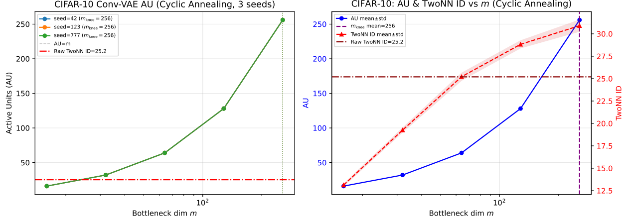
図 13: Exp-Nat-Cifar: m -dependence of AU and TwoNN ID for CIFAR-10 Conv-VAE (KL cyclic annealing, 3 seeds). TwoNN ID shows convergence consistent with Pope et al.[17] ( d_{ID} \approx 26 ). (Note: axis labels to be updated to English in final submission.)
