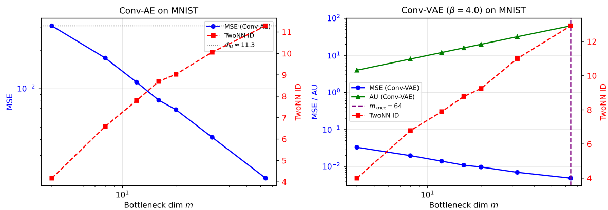
図 10: Exp-Conv-AE: m -dependence of MSE, AU, and TwoNN ID for MNIST Conv-AE (left) and Conv-VAE (right) (100 epochs). Conv-AE confirms AU = m (all dims active) with TwoNN ID converging to \approx 11 at m \geq 32 . Conv-VAE shows AU \approx m (no saturation due to insufficient convergence at 100 epochs). (Note: axis labels to be updated to English in final submission.)
