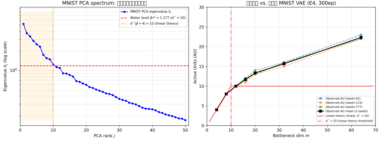
図 7: Exp-Mnist-PCA: (Left) MNIST PCA eigenvalue spectrum and linear-theory water-filling level ( \beta\tau^2 \approx 1.18 , d^* = 10 ). (Right) Comparison of linear theory prediction (red solid line; sharp saturation assumed at d^* = 10 ) and observed AU( m ) curve of nonlinear FC-VAE (per seed and mean). The gradual AU increase in the nonlinear VAE provides the theoretical basis for m^{\text{knee}} instability. (Note: axis labels to be updated to English in final submission.)
