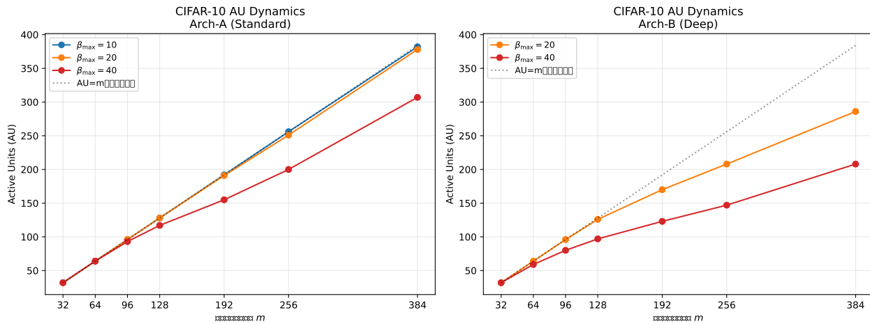
図 15: Exp-NatImg-AU: AU dynamics of CIFAR-10 Conv-VAE. (Left) Arch-A (Standard), (Right) Arch-B (Deep). Dotted line: \text{AU} = m reference (no saturation). Increasing \beta_{\text{max}} strengthens AU suppression, but no saturation plateau is reached under any condition. (Note: axis labels to be updated to English in final submission.)
