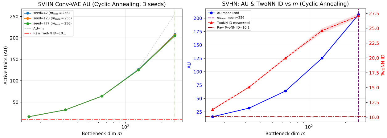
図 14: Exp-Nat-SVHN: m -dependence of AU and TwoNN ID for SVHN Conv-VAE (KL cyclic annealing, 3 seeds).
