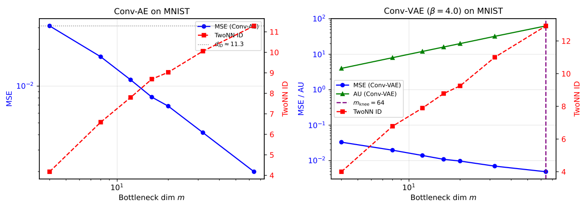
図 10: Exp-Conv-AE: m -dependence of MSE, AU, and TwoNN ID for MNIST Conv-AE (left) and Conv-VAE (right) (100 epochs). Conv-AE confirms \text{AU} = m (all dims active) with TwoNN ID converging to \approx 11 at m \geq 32 . Conv-VAE shows \text{AU} \approx m (no saturation due to insufficient convergence at 100 epochs).
