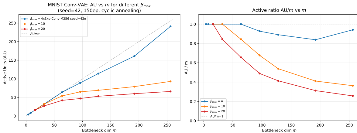
図 12: Exp-ConvV-HiBeta: Comparison of MNIST Conv-VAE AU vs m (left) and activation rate \text{AU}/m (right) for \beta_{\text{max}} \in \{4, 10, 20\} . Increasing \beta_{\text{max}} shifts AU saturation to lower dimensions, demonstrating the \beta -dependence of d^*(\beta) .
