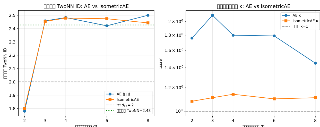
図 3: Exp-Iso-ID: (Left) Latent-space TwoNN ID by m — curves for standard AE and IsometricAE nearly overlap, showing that isometry improvement has minimal effect on TwoNN ID; (Right) Comparison of decoder condition number \kappa — IsometricAE maintains \kappa \approx 1.1 across all m , while AE rises to \kappa = 2.10 at m = 3 .
