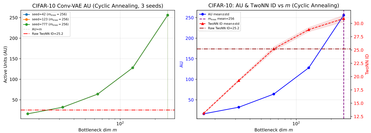
図 13: Exp-Nat-Cifar: m -dependence of AU and TwoNN ID for CIFAR-10 Conv-VAE (KL cyclic annealing, 3 seeds). TwoNN ID shows convergence consistent with Pope et al.[17] ( d_{\text{ID}} \approx 26 ).
