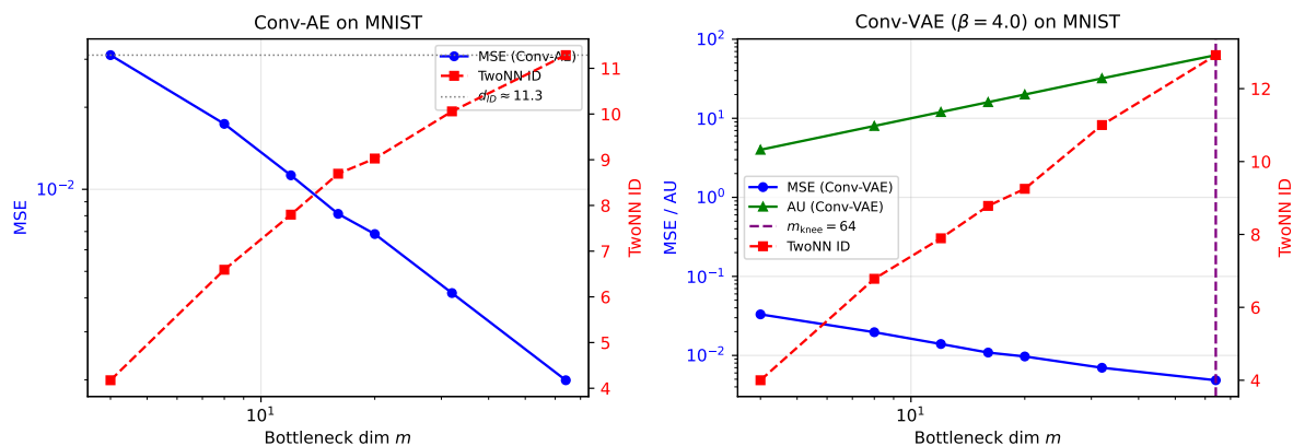
図 8: Exp-Conv-AE: m -dependence of MSE, AU, and TwoNN ID for MNIST Conv-AE (left) and Conv-VAE (right) (100 epochs). Conv-AE confirms \text{AU} = m (all dims active) with TwoNN ID converging to \approx 11 at m \geq 32 . Conv-VAE shows \text{AU} \approx m (no saturation due to insufficient convergence at 100 epochs).
