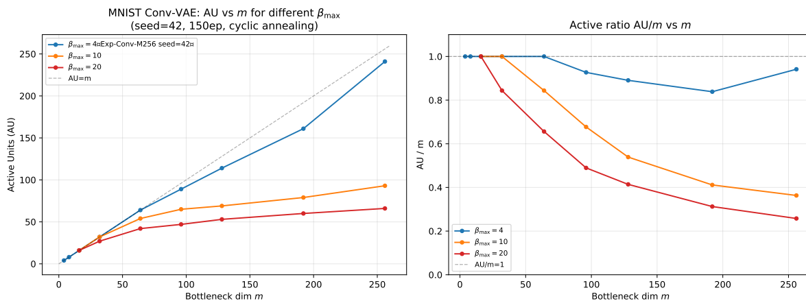
図 10: Exp-ConvV-HiBeta: Comparison of MNIST Conv-VAE AU vs m (left) and activation rate \text{AU}/m (right) for \beta_{\max} \in \{4, 10, 20\} . Increasing \beta_{\max} shifts AU saturation to lower dimensions, demonstrating the \beta -dependence of d^*(\beta) .
