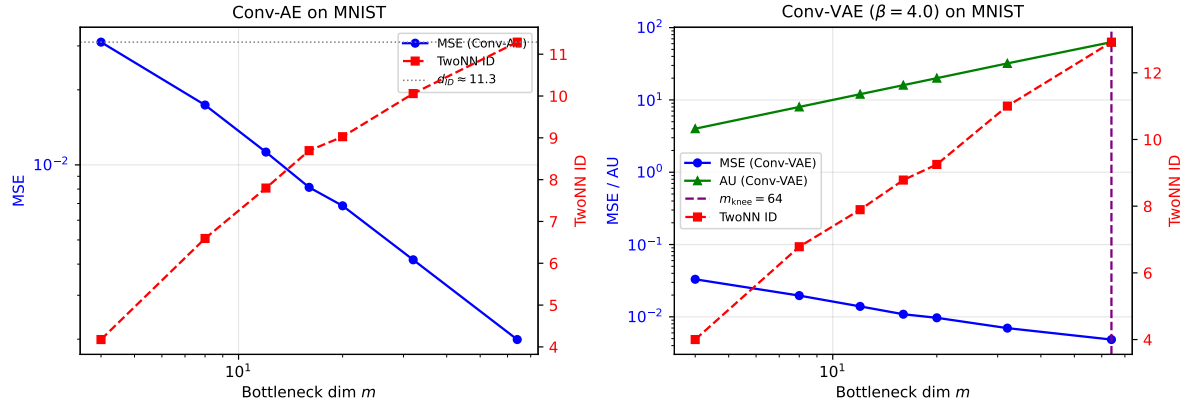
図 8: Exp-Conv-AE: m -dependence of MSE, AU, and TwoNN ID for MNIST Conv-AE (left) and Conv-VAE (right) (100 epochs). Conv-AE confirms AU = m (all dims active) with TwoNN ID converging to \approx 11 at m \geq 32 . Conv-VAE shows AU \approx m (no saturation due to insufficient convergence at 100 epochs).
