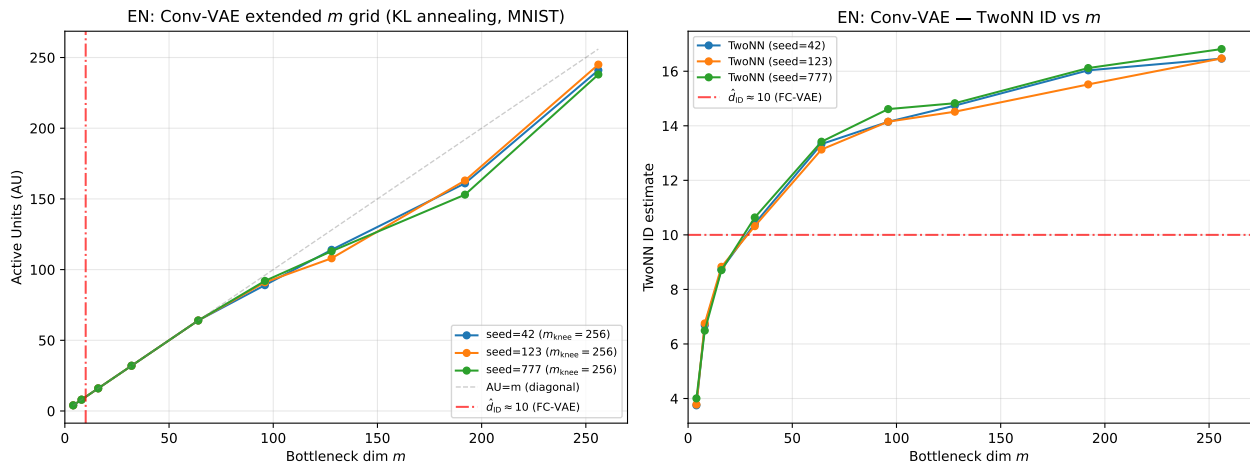
図 9: Exp-Conv-M256: Conv-VAE extended m grid ( m \in [4, 256] , KL annealing, 3 seeds). AU vs m (left) and TwoNN ID vs m (right). Diagonal line (AU = m ) and FC-VAE reference \hat{d}_{\text{ID}} \approx 10 (red) are shown. AU = m continues at m \leq 64 but deviates from the diagonal at m \geq 96 , confirming qualitative water-filling behavior in Conv-VAE.
