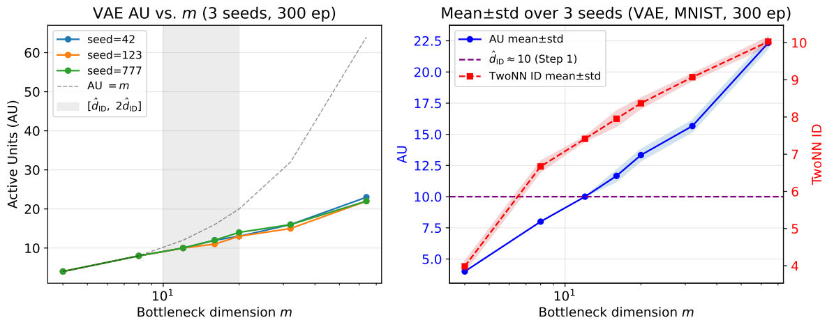
图 3: MNIST: multi-seed reproducibility of the AU verification signal (3 seeds, 300 epochs). Left: per-seed \text{AU}(m) with the ID-guided candidate range [\hat{d}_{\text{ID}}, 2\hat{d}_{\text{ID}}] shaded; right: mean \pm std band with the Step-1 reference \hat{d}_{\text{ID}} \approx 10 . AU values are highly reproducible ( \sigma \leq 0.5 ). Change-point (knee) estimates are deliberately not shown here; they are exploratory only (Appendix 付録 B).
