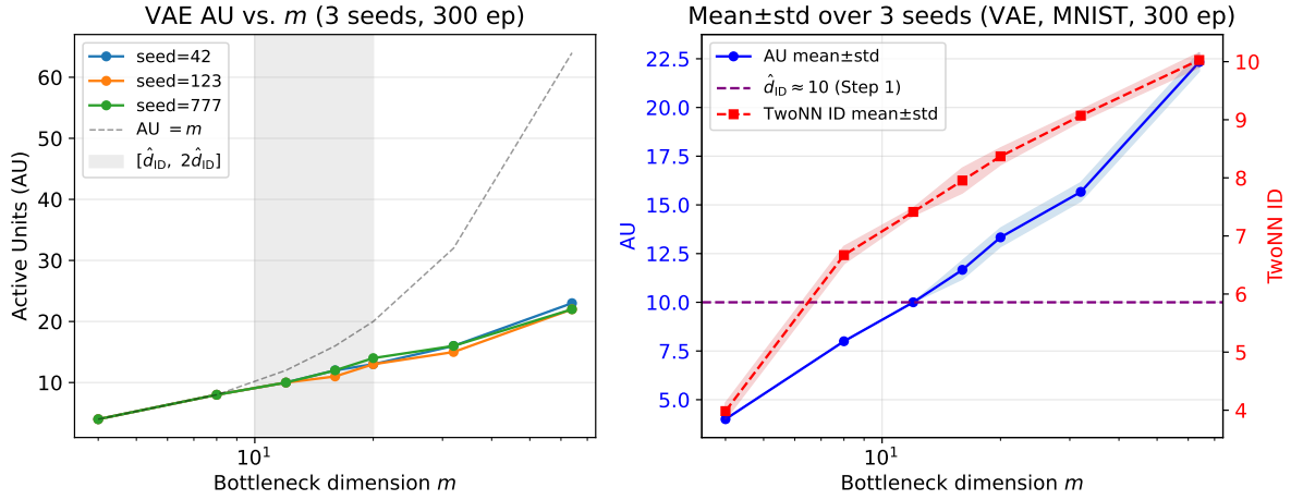
図 3: MNIST: multi-seed reproducibility of the AU verification signal (3 seeds, 300 epochs). Left: per-seed AU(m) with the ID-guided candidate range [\hat{d}_{ID}, 2\hat{d}_{ID}] shaded; right: mean±std band with the Step-1 reference \hat{d}_{ID} \approx 10 . AU values are highly reproducible ( \sigma \leq 0.5 ). Change-point (knee) estimates are deliberately not shown here; they are exploratory only (Appendix 付録 B).
