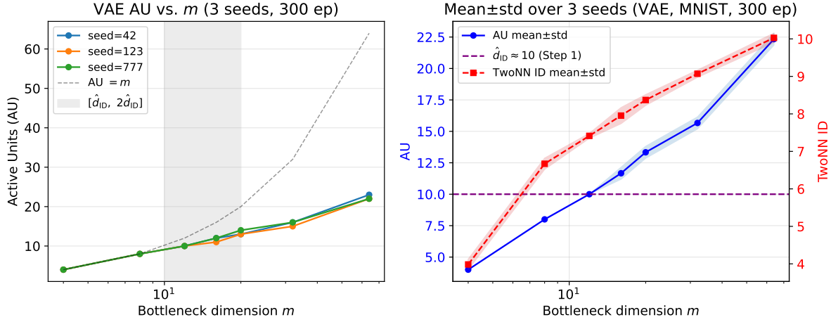
図 3: MNIST: multi-seed reproducibility of the AU verification signal (3 seeds, 300 epochs). Left: per-seed AU(m) with the ID-guided search window [\hat{d}_{ID}, 2\hat{d}_{ID}] shaded; right: mean±std band with the Step-1 reference \hat{d}_{ID} \approx 10 . AU values are highly reproducible ( \sigma \leq 0.5 ). Change-point (knee) estimates are deliberately not shown here; they are exploratory only (Appendix 付録 B).
