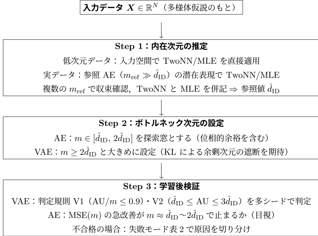
図 1: ID-guided protocol for choosing the bottleneck dimension m . The protocol closes the loop: the data-side estimate \hat{d}_{\text{ID}} determines the design, and the model-side observable AU verifies the design after training.
