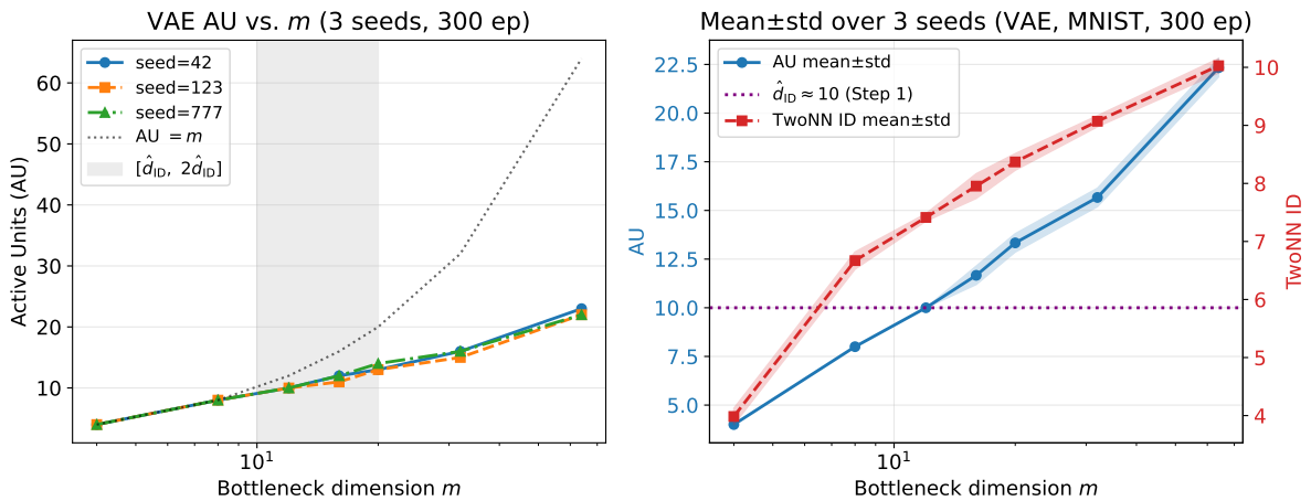
图 3: MNIST: multi-seed reproducibility of the AU verification signal (3 seeds, 300 epochs). Left: per-seed AU( m ) with the ID-guided search window [\hat{d}_{\text{ID}}, 2\hat{d}_{\text{ID}}] shaded; right: mean \pm std band with the Step-1 reference \hat{d}_{\text{ID}} \approx 10 . AU values are highly reproducible ( \sigma \leq 0.5 ). Change-point (knee) estimates are deliberately not shown here; they are exploratory only (Appendix 付録 B).
