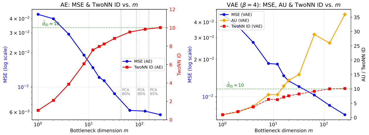
图 2: MNIST: m -dependence of the indicators (300 epochs). Left (AE) : MSE (log scale, left axis) and TwoNN ID (right axis); vertical dotted lines mark the PCA 80/90/95% dimensions (43/86/152), far above the nonlinear estimate \hat{d}_{\text{ID}} \approx 10 . Right (VAE, \beta = 4 ) : MSE, AU, and TwoNN ID; the AU growth slows beyond m \approx \hat{d}_{\text{ID}} .
