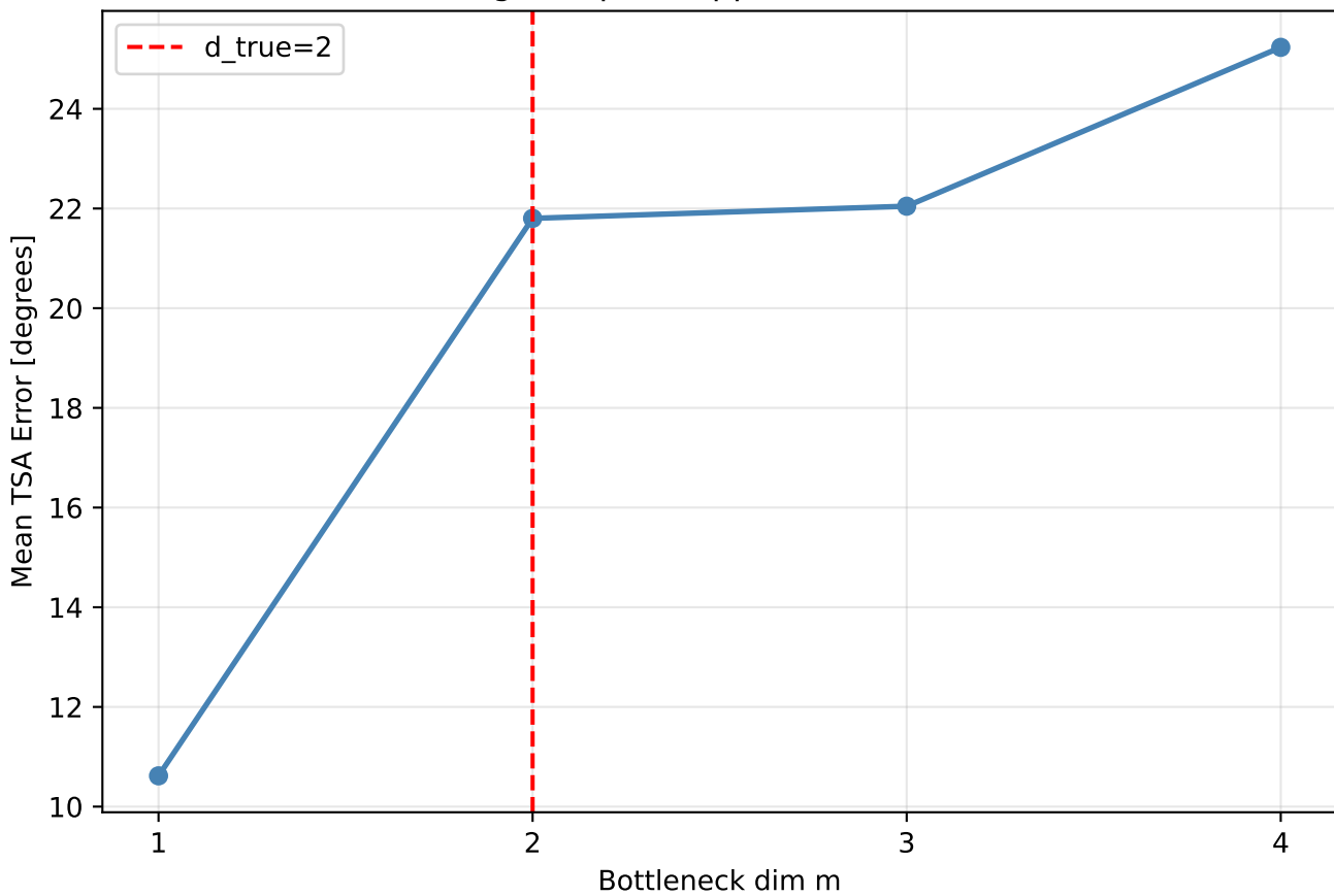
Torus: Tangent Space Approximation Error vs m
