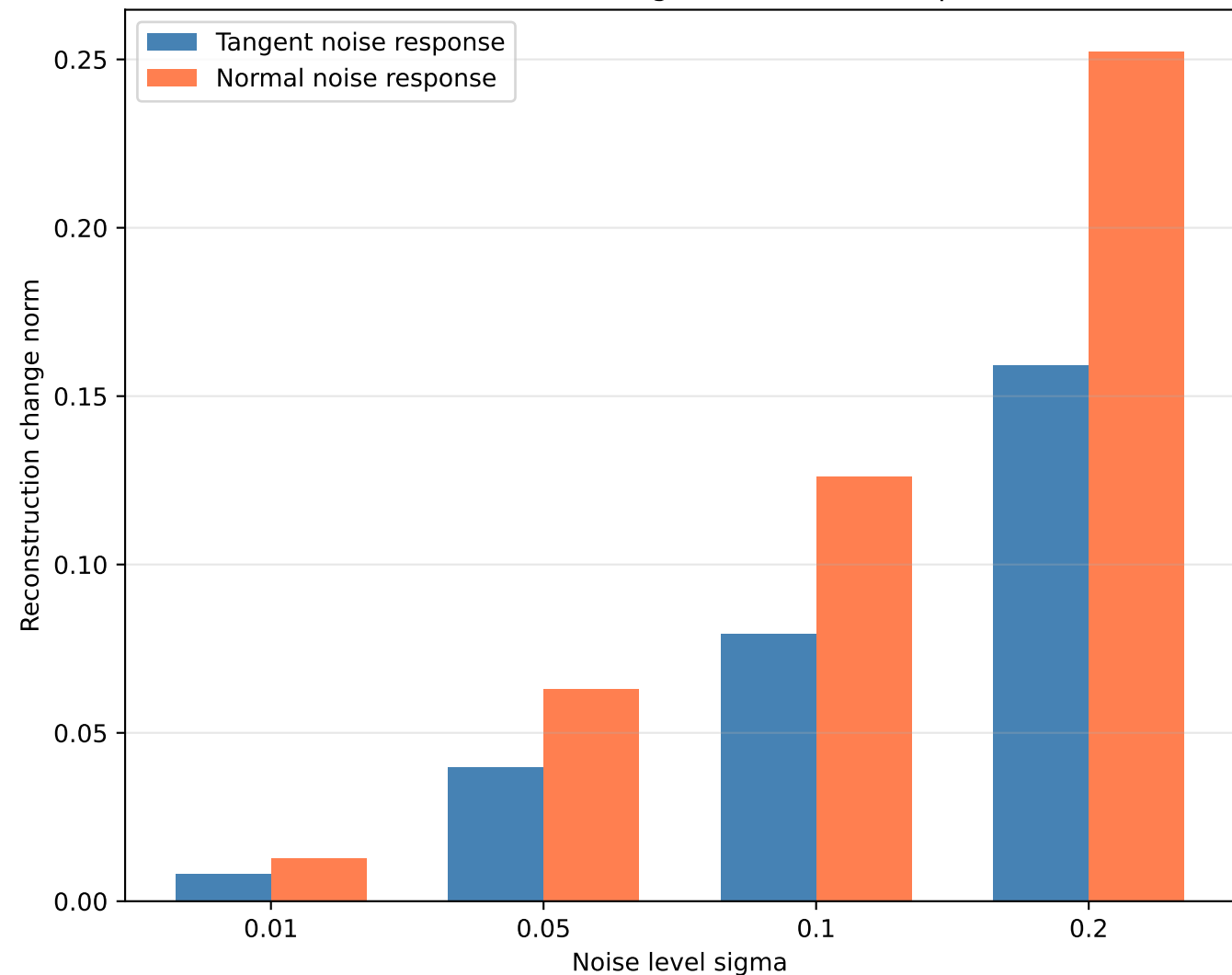
Swiss Roll ( m=2 ): Tangent vs Normal Response
