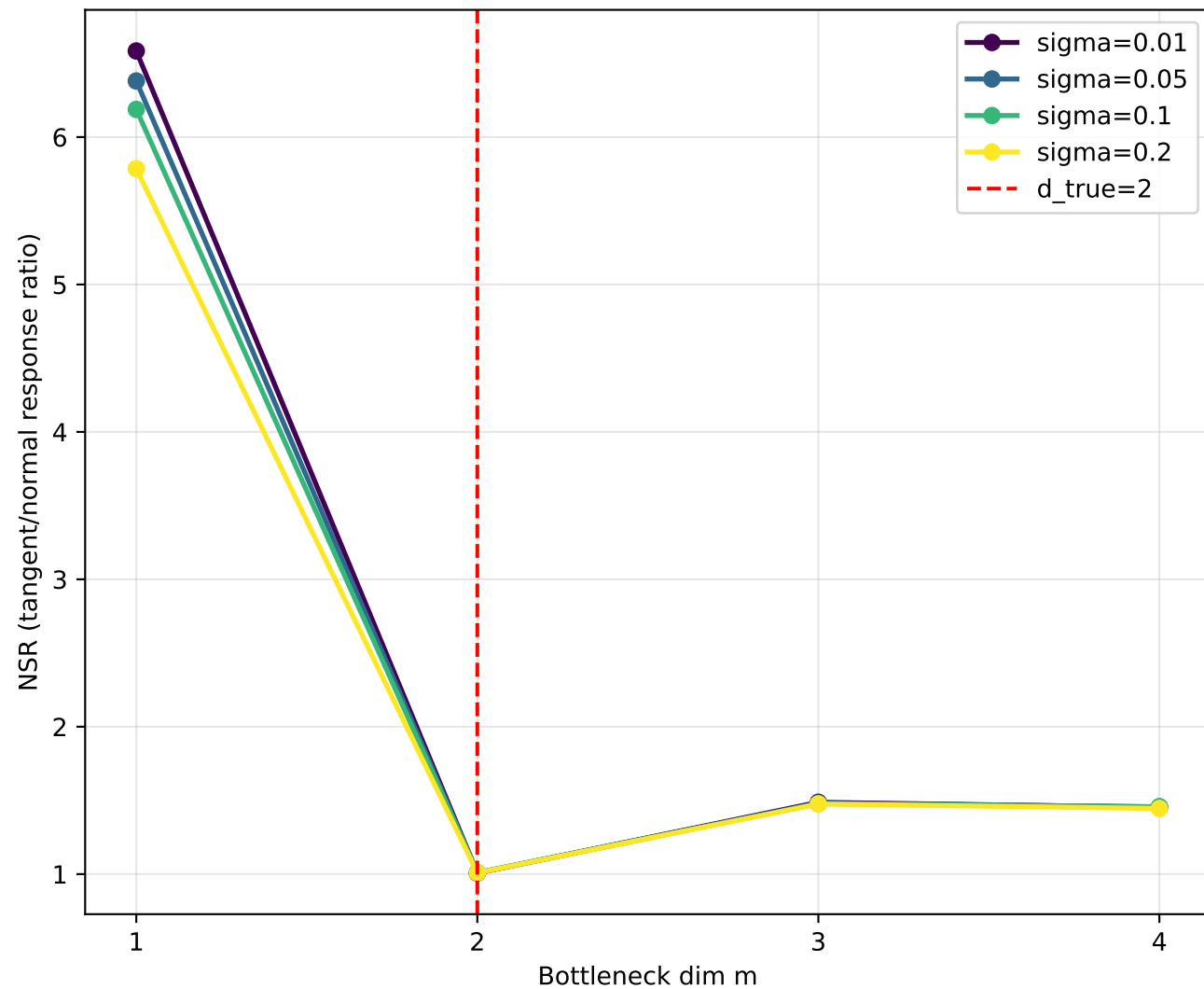
Swiss Roll: NSR vs m
