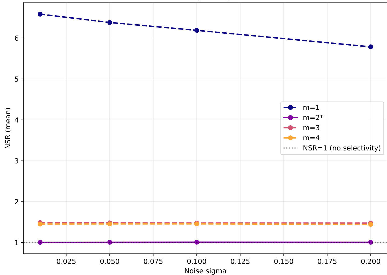
Swiss Roll: NSR vs sigma (by bottleneck dim)
