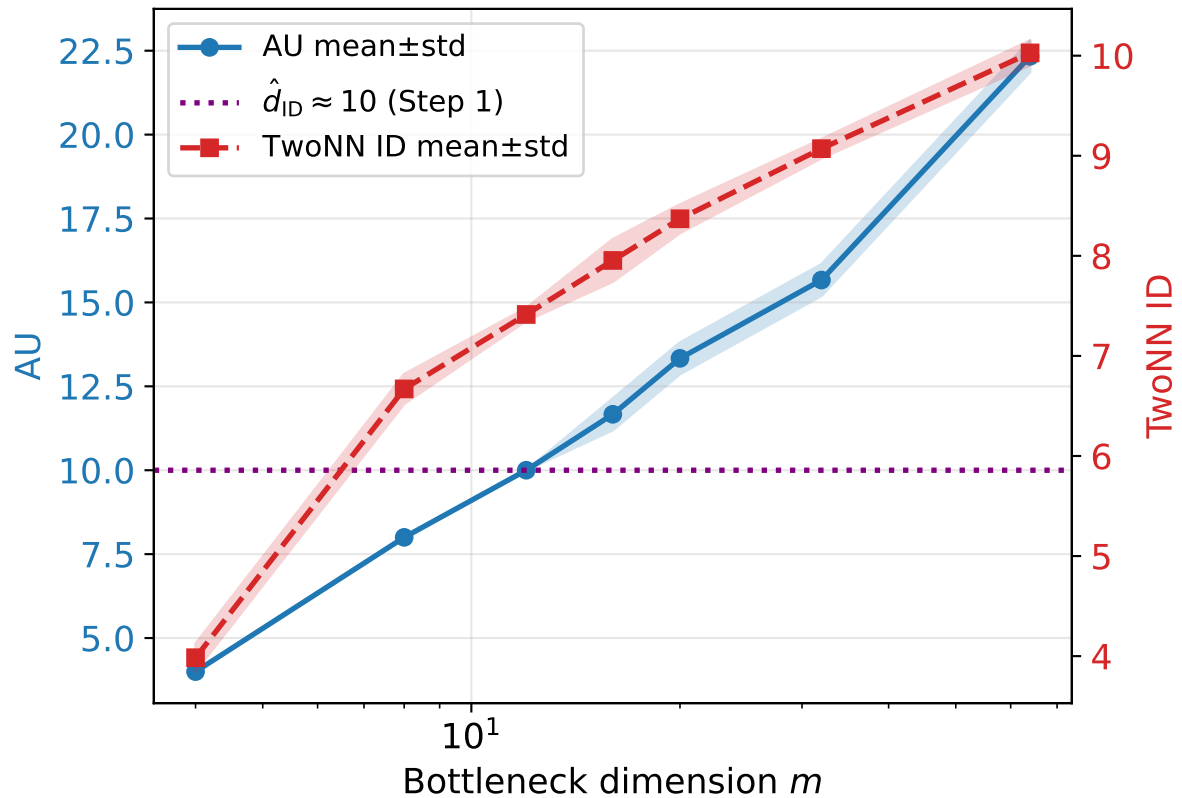
Mean \pm std over 3 seeds (VAE, MNIST, 300 ep)
