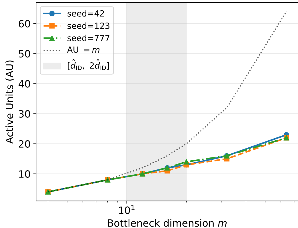
VAE AU vs. m (3 seeds, 300 ep)
