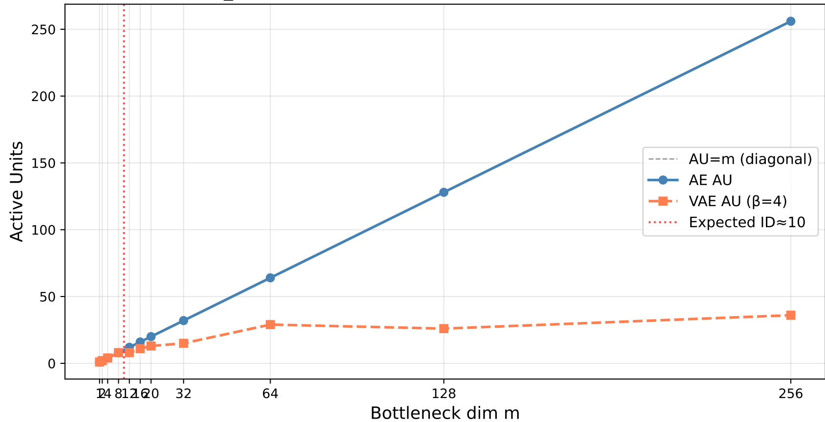
E4_extended: Active Units vs Bottleneck Dim (MNIST)
