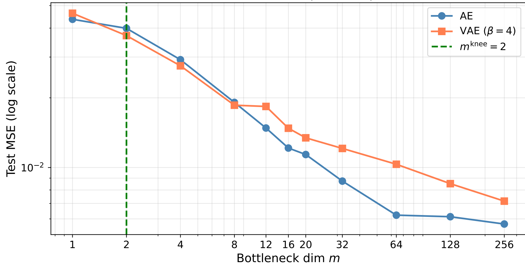
E4: MNIST Metric Sweeps (300 epochs)
