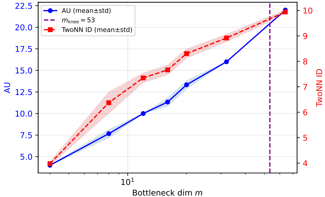
Mean \pm Std over 3 seeds (VAE, MNIST)
