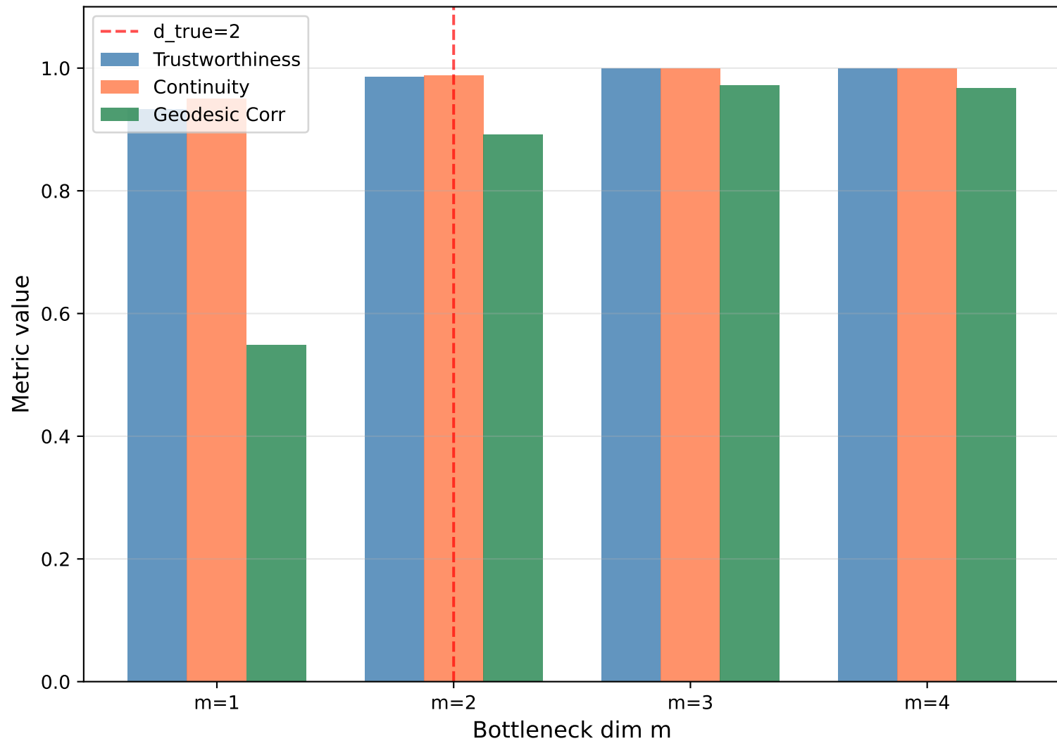
Torus: Structure Metrics vs m
