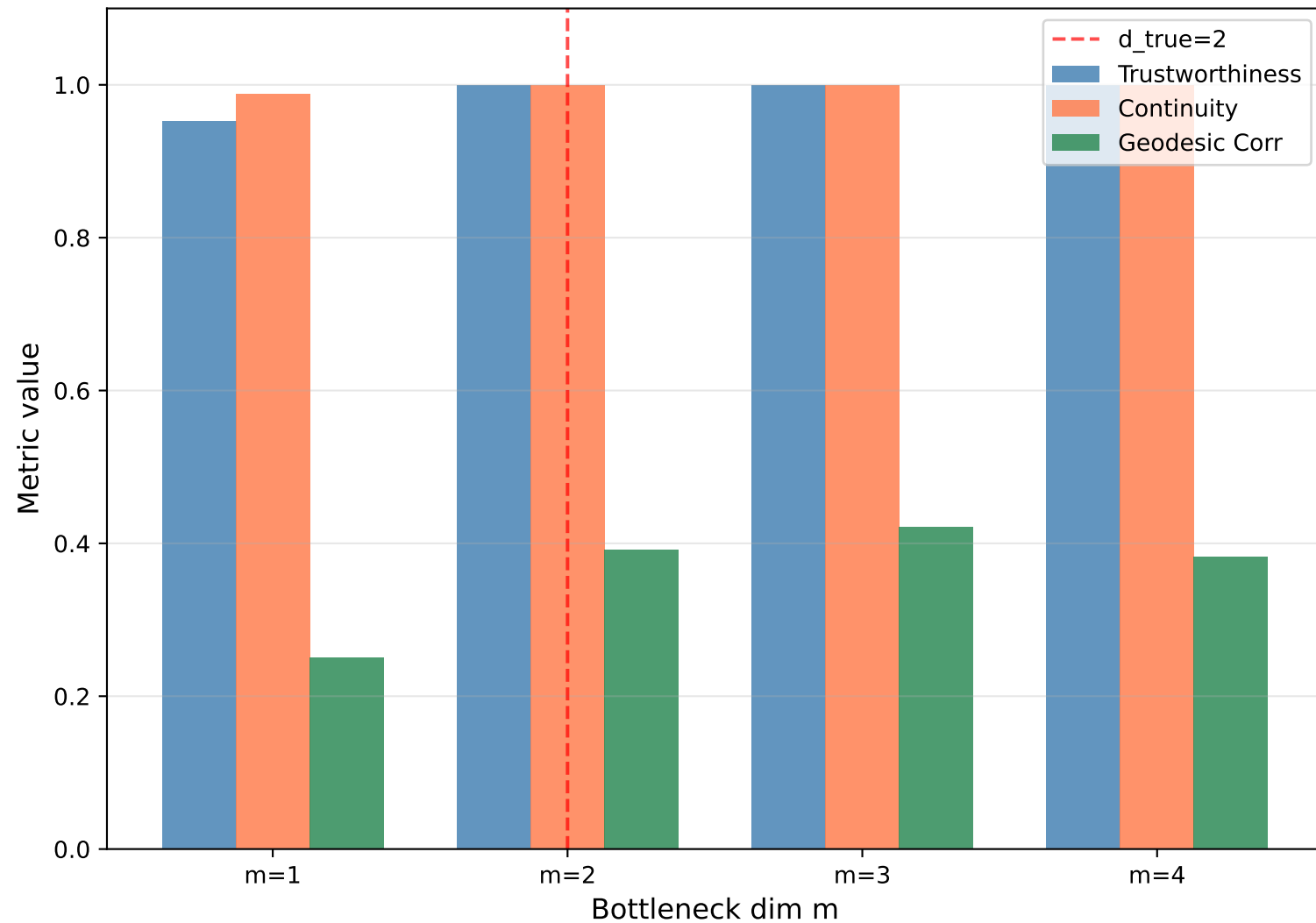
SwissRoll: Structure Metrics vs m
