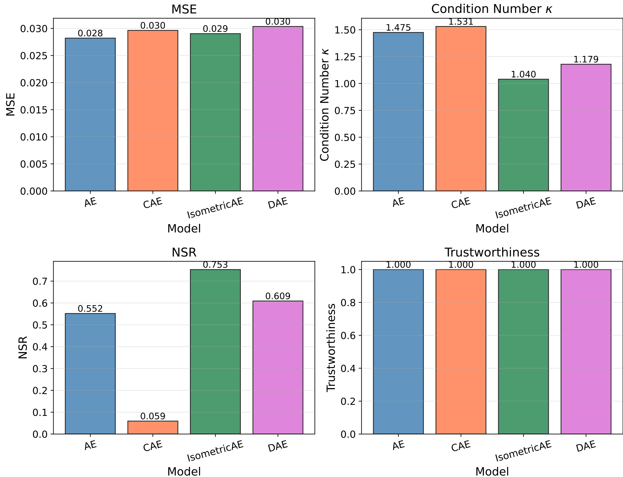
EC: AE Variant Comparison on Swiss Roll ( m = 2 )
