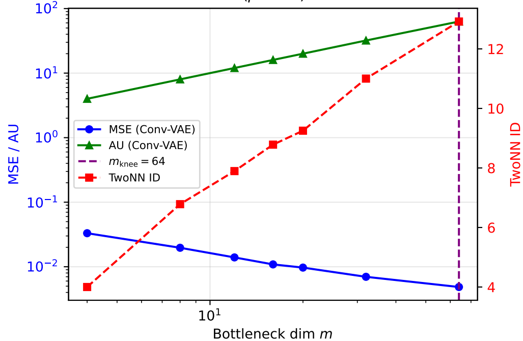
Conv-VAE ( \beta = 4.0 ) on MNIST
