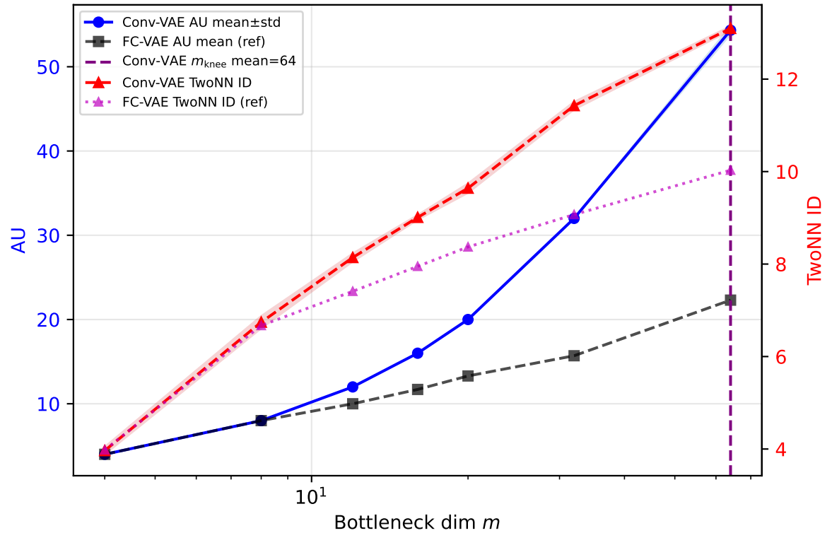
Conv-VAE vs FC-VAE (300 ep, MNIST)
