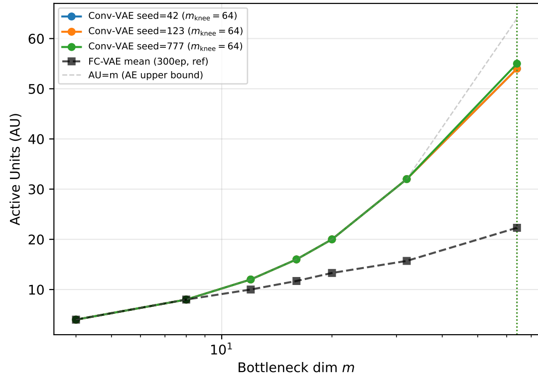
Conv-VAE AU vs m (3 seeds, 300 ep)
