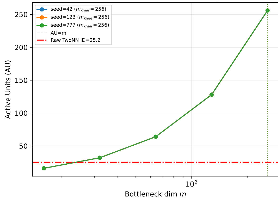
CIFAR-10 Conv-VAE AU (Cyclic Annealing, 3 seeds)
