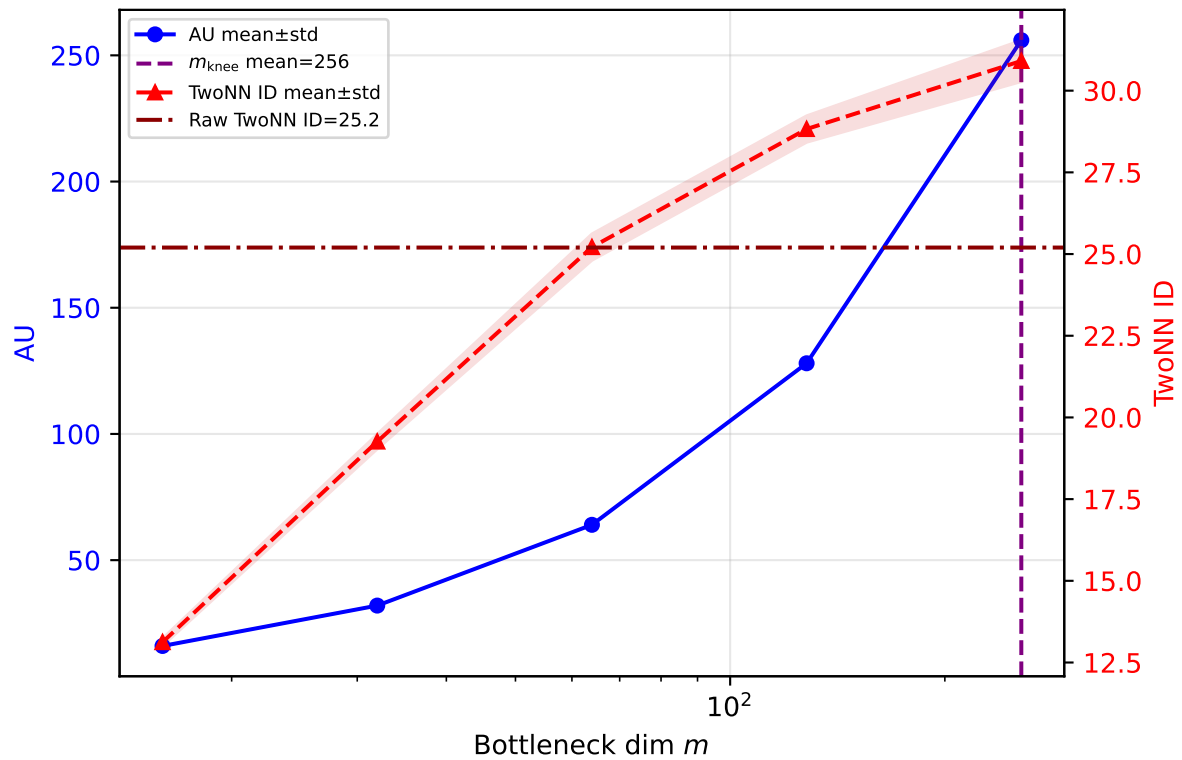
CIFAR-10: AU & TwoNN ID vs m (Cyclic Annealing)
