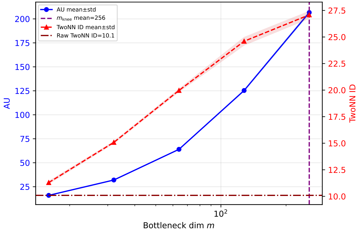
SVHN: AU & TwoNN ID vs m (Cyclic Annealing)
