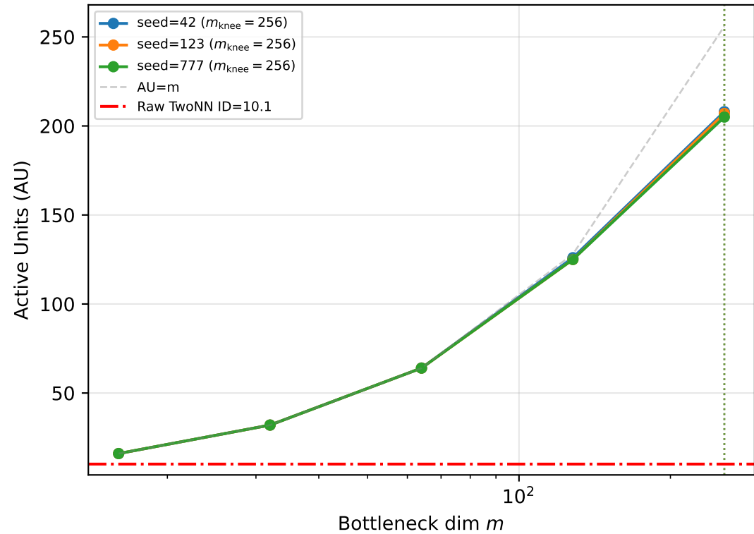
SVHN Conv-VAE AU (Cyclic Annealing, 3 seeds)
