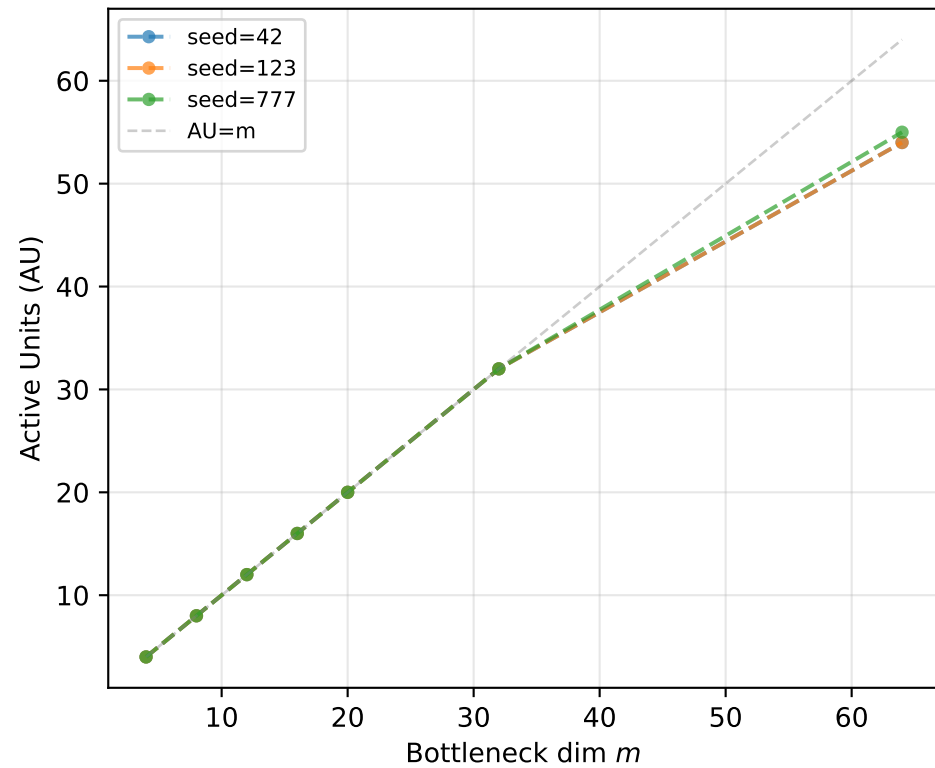
Fixed \beta=4.0 (EH)
