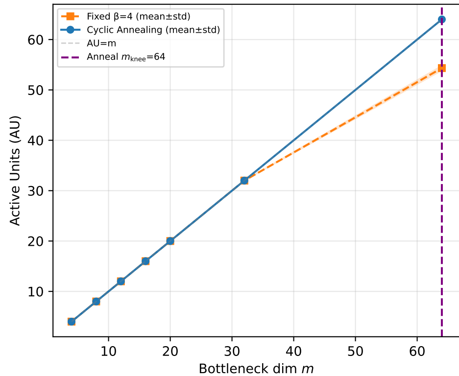
Fixed \beta vs KL Annealing: AU comparison
