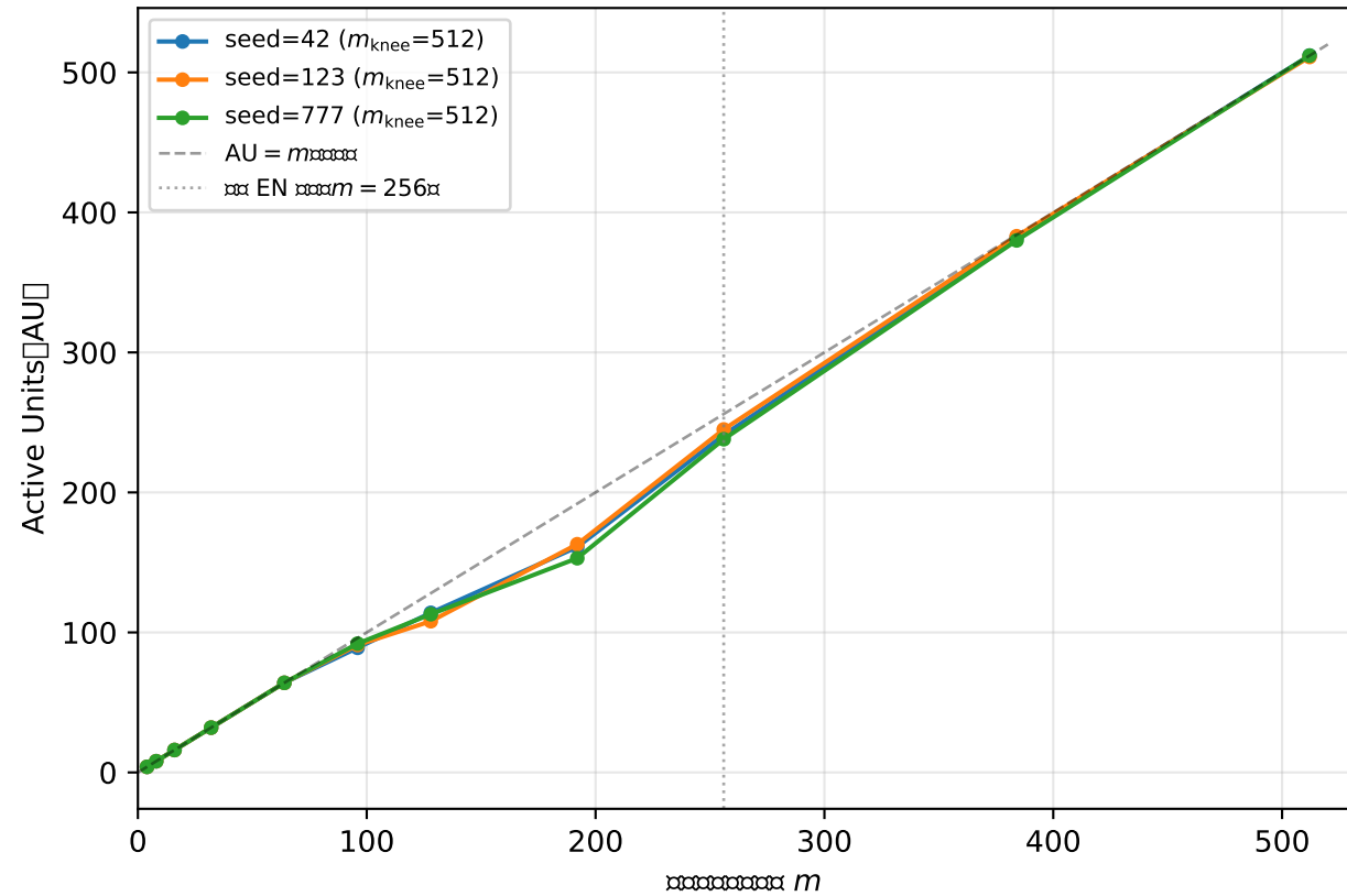
EN_ext: MNIST Conv-VAE AU vs m m \leq 512 \beta_{\max} = 4
