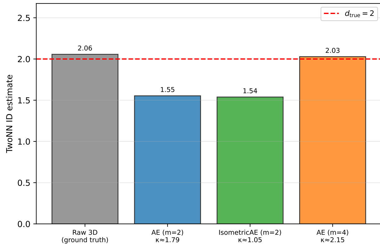
Section A: Swiss Roll — TwoNN by model (effect of \kappa ) ( d_{\text{true}} = 2 , 3D input)
