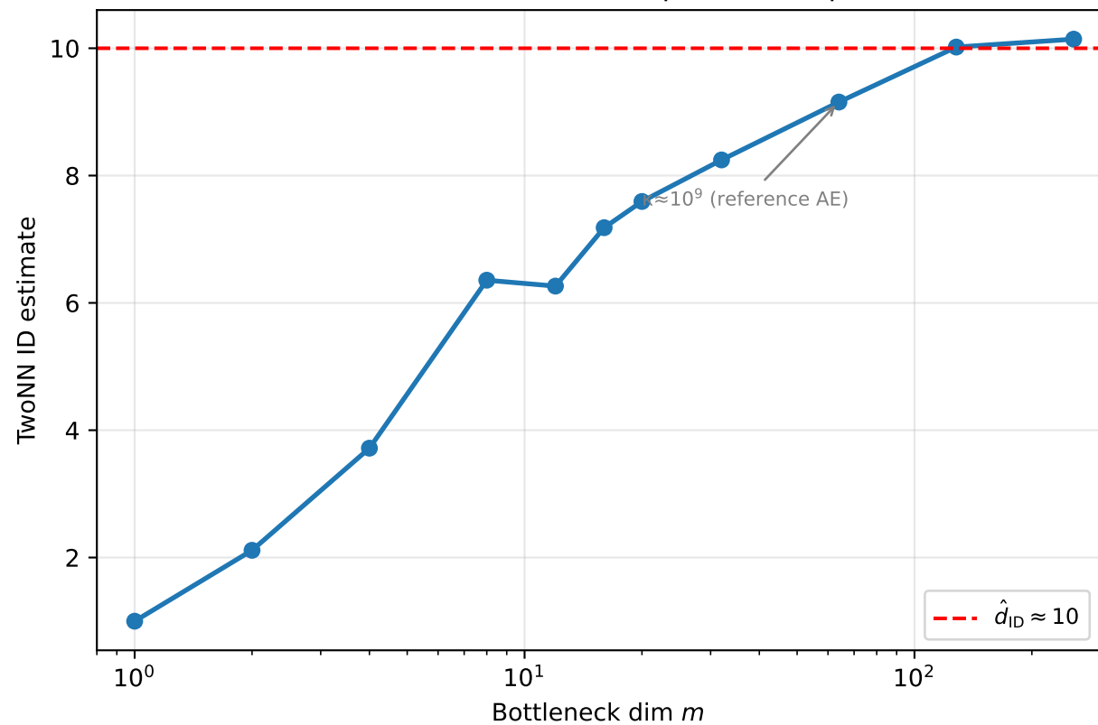
Section B: MNIST — TwoNN convergence vs m (reference AE, \kappa \approx 10^9 ; \beta = 4 , 300ep)
